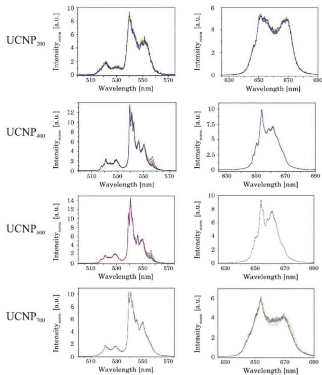
Fig. 11 TRANES of annealed UCNPs ( 200 \text{ }^\circ\text{C} < x < 700 \text{ }^\circ\text{C} ) for (left) G1 and G2 luminescence as well as (right) of R luminescence are shown ( \lambda_{\text{ex}} = 976 \text{ nm} ). The delay after the laser pulse was varied between 0 \mu\text{s} and 2000 \mu\text{s} .
