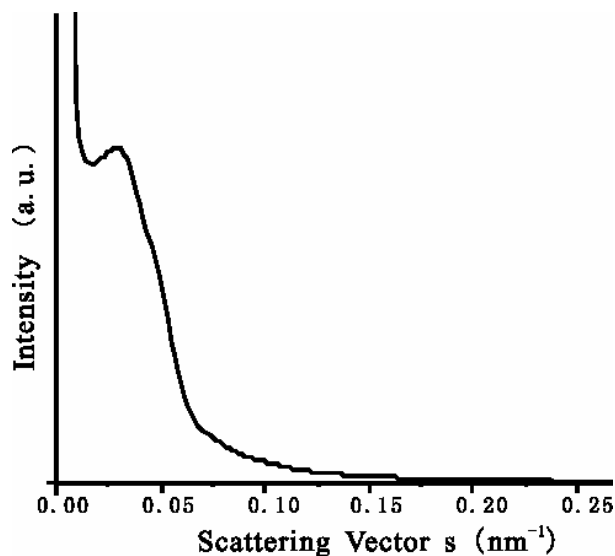
Figure 4.10 SAXS pattern of sample B-Ti-PP.
