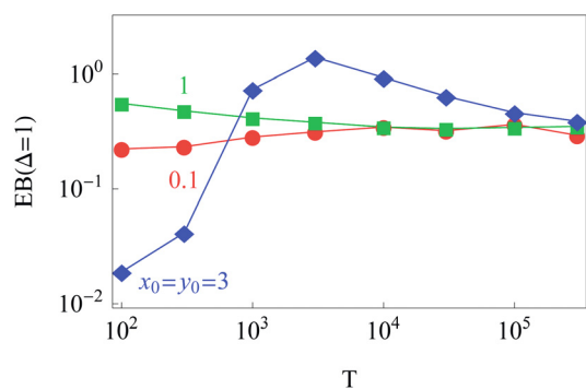
Fig. 6 Dependence of EB(\Delta = 1) on the trace length T . At least N = 300 trajectories were used to compute each point in the graph, except for the longest trajectory, for which N = 50 . Parameters are the same as in Fig. 2.
