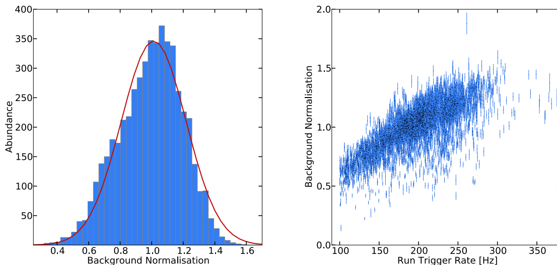
Figure 5.11.: Left : The distribution of the fitted scaling parameter of off-runs. The red line denotes a fit with a Gaussian function. Right : Background normalisation plotted versus the corresponding trigger rate of the run. The sudden cut at 100 Hz originates from the applied run selection.
