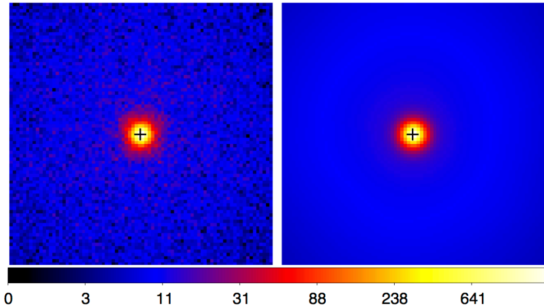
Figure 5.14.: Left : Count map of VHE \gamma -ray candidates filled from 207 runs. Right : Corresponding model map, representing the number of counts predicted by the best-fit model. Both maps show a 2^\circ \times 2^\circ region around the Crab Nebula position, which is marked by a black cross. To accommodate the strong source, the colour scale, depicting the number of VHE \gamma -ray candidates per bin, is logarithmically stretched.
