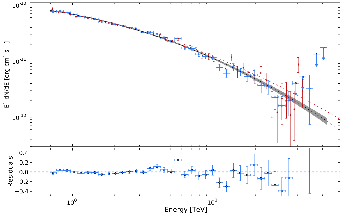
Figure 5.16.: SED of the Crab Nebula, derived with GAMMALIB and the H. E. S. S. software. The blue points denote the spectral points derived in the likelihood framework of GAMMALIB. The black-dashed line represents the corresponding best-fit model. The grey-shaded area depicts the corresponding 68% confidence region. The red-dashed line shows the best-fit model, derived with the H. E. S. S. software. The lower panel depicts the residuals from the data point with respect to the best-fit model.
