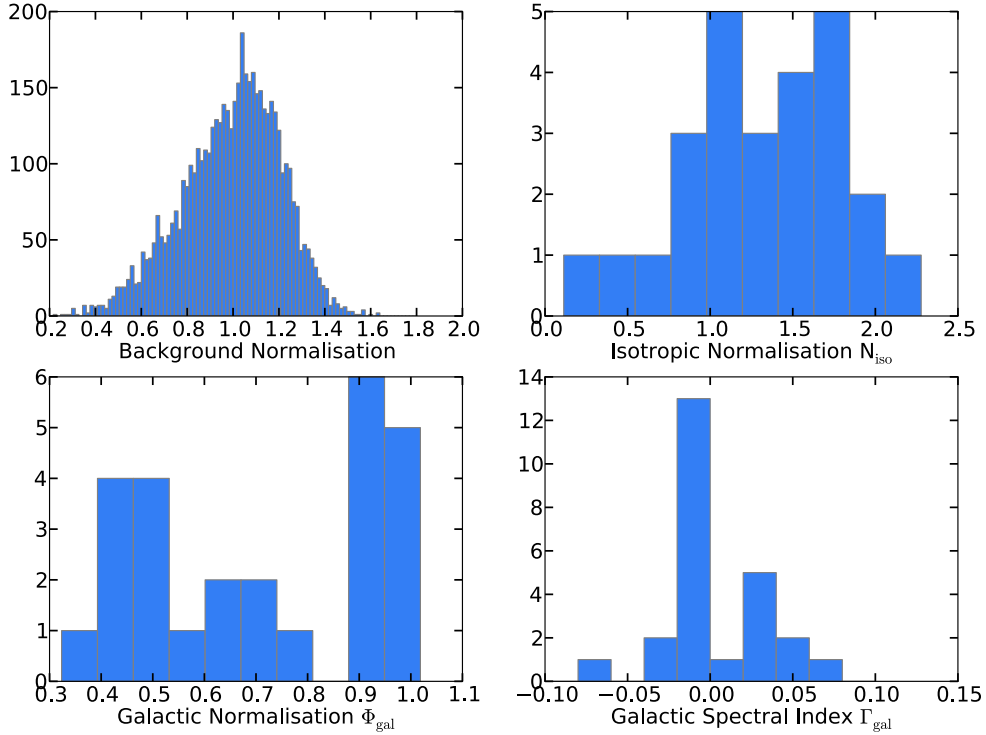
Figure 5.23.: The four panels represent the distribution of the background parameter, fitted in the combined analyses of PWNe. Top left : Background normalisation factor of all analysed H. E. S. S. runs. Top right : Normalisation of the Fermi -LAT isotropic diffuse component. Bottom left : The scaling prefactor of the Galactic diffuse model for Fermi -LAT. Bottom right : Distribution of the spectral index, which additionally scales the energy dependence of the Galactic diffuse model.
