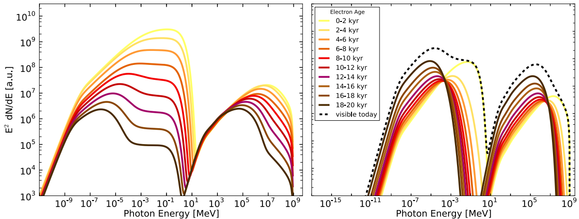
Figure 2.4.: SED evolution and composition of a generic PWN as predicted by the model. The used parameters follow the column “mean model” in Table 2.1. Left : Time evolution of the SED, ranging from a young (0.5 kyr, yellow) to an old (150 kyr, dark red) PWN. Right : The SED of a 20 kyr old PWN shown as black-dashed line. Coloured lines denote a decomposition of the SED into contributions by electrons from different injection epochs.
