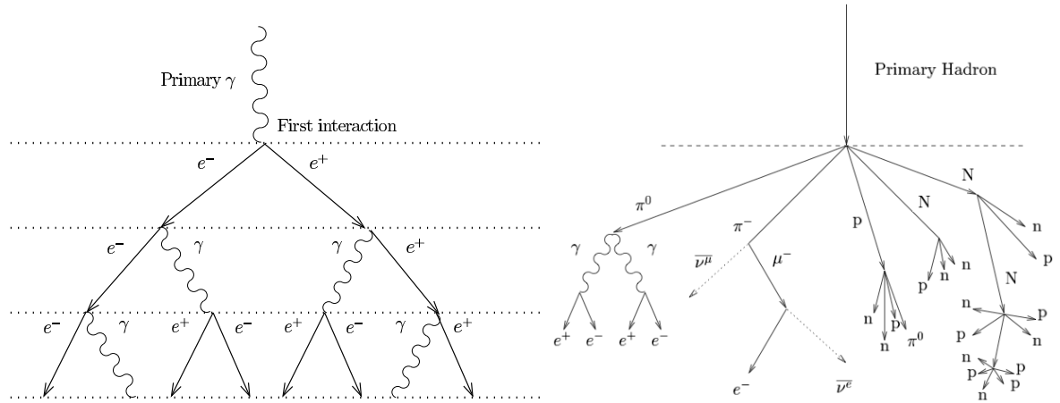
Figure 5.1.: Left : Schematic illustration of an air shower, induced by a \gamma -ray hitting the atmosphere. The distances between the horizontal dotted lines represent one radiation length. Right : Scheme of a hadron-induced air shower, showing several sub-showers, among others an electromagnetic one on the very left. The particles p and n represent nucleons created in hadronic interactions, while N stands for an energetic atomic nucleus. Further shown are pions ( \pi^{\pm,0} ), neutrinos ( \nu ) and muons ( \mu ). Both images are adopted from Funk (2005).
