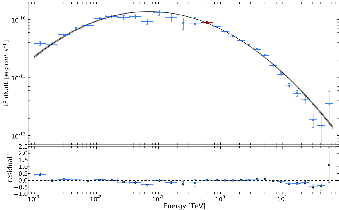
Figure 5.20.: The top panel presents the result of the first combined analysis of Fermi -LAT and H. E. S. S. data. The grey-shaded band depicts the 68% confidence region of the spectral fit with a log-parabola model over almost five decades in energy. The blue points result from spectral fits in energy bands. The data point highlighted in red depicts the one energy bin, where both instruments contribute. The bottom panel represents the residuals from the data points with respect to the best-fit model.
