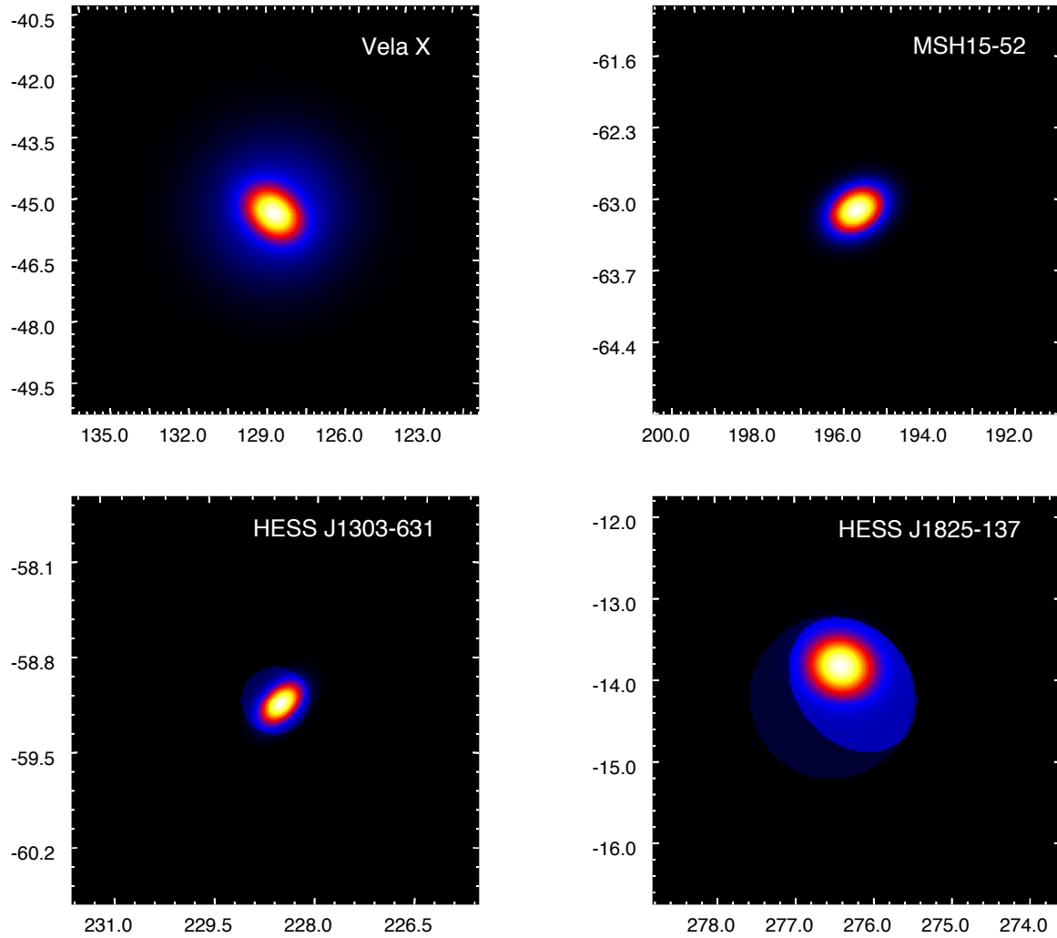
Figure A.5.: The templates used for PWNe with complex morphologies. Note that each map has a different size in the sky. The coordinates indicate Right Ascension and Declination in units of degrees.
