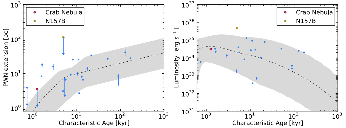
Figure 2.6.: Left : The intrinsic size of the considered PWNe (blue points) plotted versus the characteristic age of the associated pulsar. Overlaid as grey-shaded area is the model prediction from Eq. 2.18 with the artificial spread listed in Table 2.1. The black-dashed line denotes the “mean model”. Right : Intrinsic PWN luminosity between 1 – 10 TeV also shown against the characteristic age. The modelled solid line is also based on the predicted evolution by the “mean model”, while the grey-shaded area mimics an intrinsic scatter.
