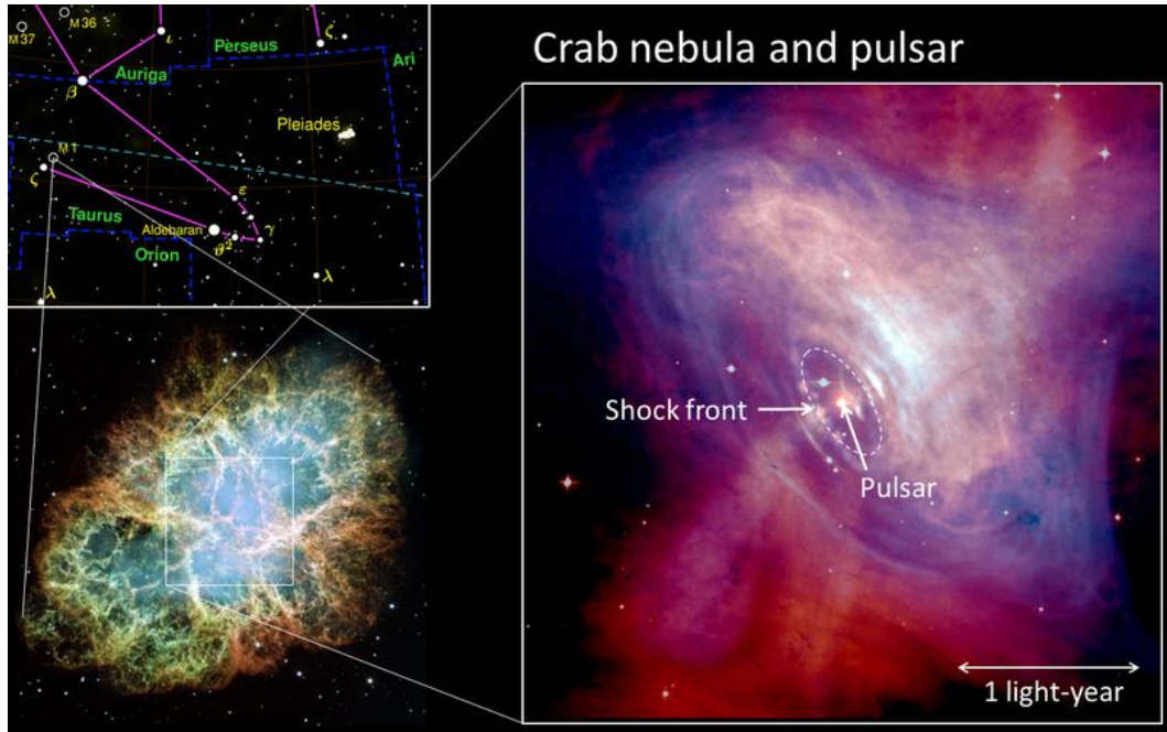
Figure 2.1.: Several views on the Crab Nebula. Top left: The position of the Crab Nebula with respect to other bright stars in the Taurus region. Lower left: The Crab Nebula in optical wavelengths imaged by the Hubble Space Telescope. Right: The X-ray emission from the central region, measured by the Chandra X-ray Observatory. The Crab pulsar can be clearly recognised as bright point source in the image center. Image credit: Composition: MPIK, Pictures: NASA
