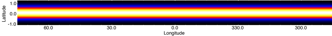
Figure 5.22.: Gaussian band model in Galactic coordinates, mimicking the Galactic diffuse emission in the H. E. S. S. energy range. The colour scale is linear from low intensities (dark) to high intensities (bright).
