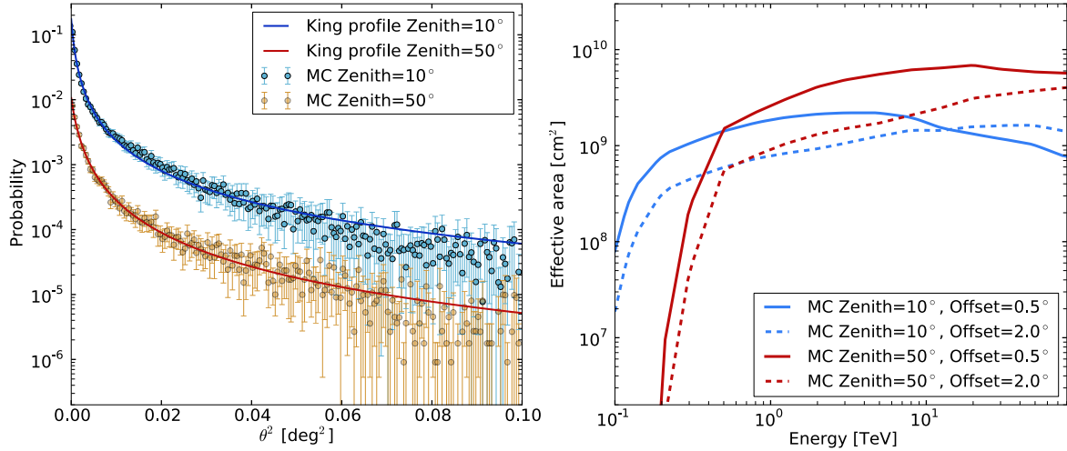
Figure 5.6.: PSF and A_{\text{eff}} for H. E. S. S., derived for a fixed azimuth of 0^\circ and muon efficiency of 100%. Left : Shape of the PSF with squared offset from the true source position, which is simulated at an offset of 0.5^\circ from the telescope pointing position. The data points correspond to the respective MC simulation, while the lines present the fit of a King profile (Eq. 5.3) to the data. Note that the distributions for the zenith angle of 50^\circ (orange/red) are scaled down by a factor of ten for improved visibility. Right : The H. E. S. S. effective area as a function of energy. As indicated in the legend on the lower right, the different curves represent four setting of MC simulations.
