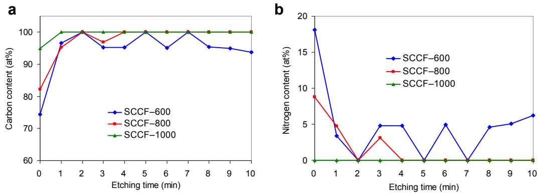
Figure 4–8 Depth profiles for the films by X-ray photoelectron spectroscopy (XPS).
