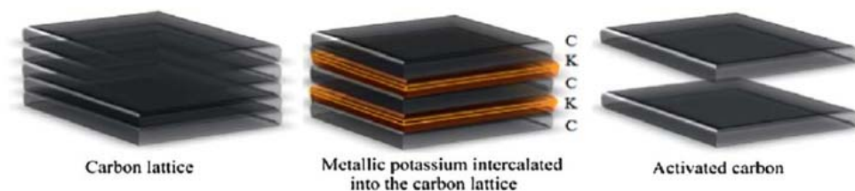
Figure 1–6 Activation mechanism using potassium hydroxide (KOH). [54]
