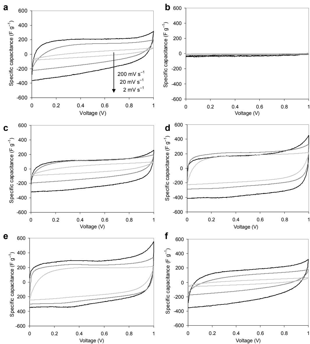
Figure 2–15 Cyclic voltammetry charts for the Cs salt-flux carbons in H_2SO_4 at the sweep rate of 2, 20 and 200 mV s^{-1} .
