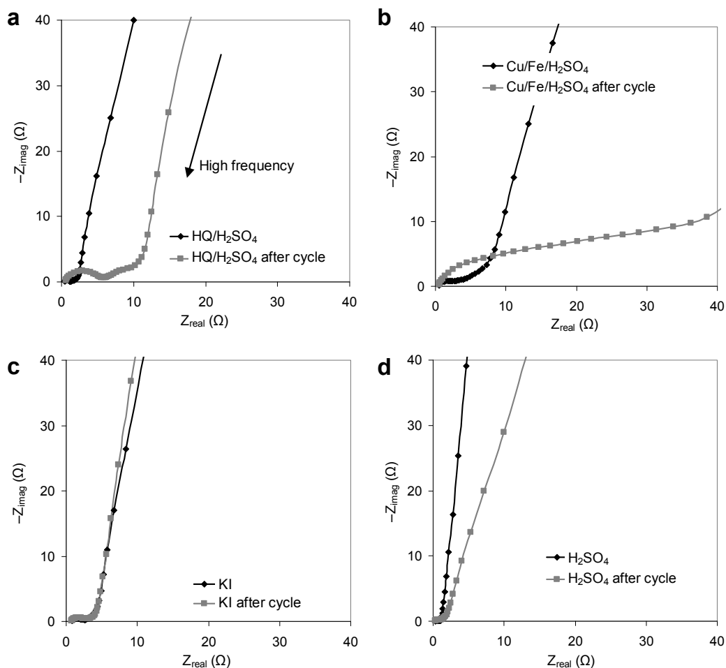
Figure 3–8 Nyquist plots for before and after the cycle stability test (2500 times at 2 A g -1 ) of SFC–9.
