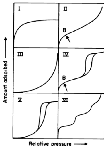
Figure 6–2 Types of physisorption isotherms. [181]
