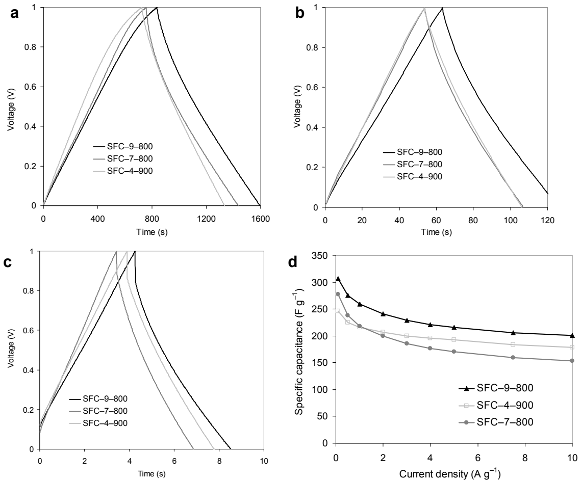
Figure 2-20 Galvanostatic charge/discharge profiles for the Cs salt-flux carbons in KOH.
