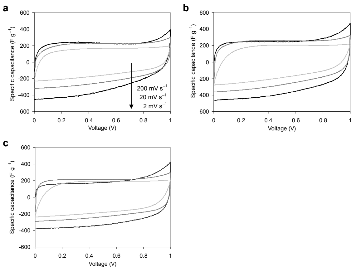
Figure 2–19 Cyclic voltammetry charts for the Cs salt-flux carbons in KOH at the sweep rate of 2, 20 and 200 \text{ mV s}^{-1} .
