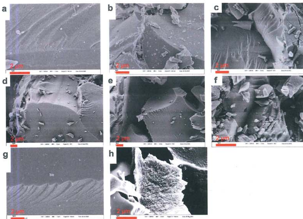
Figure 2-11 Scanning electron micrographs (magnification) for the carbons.
