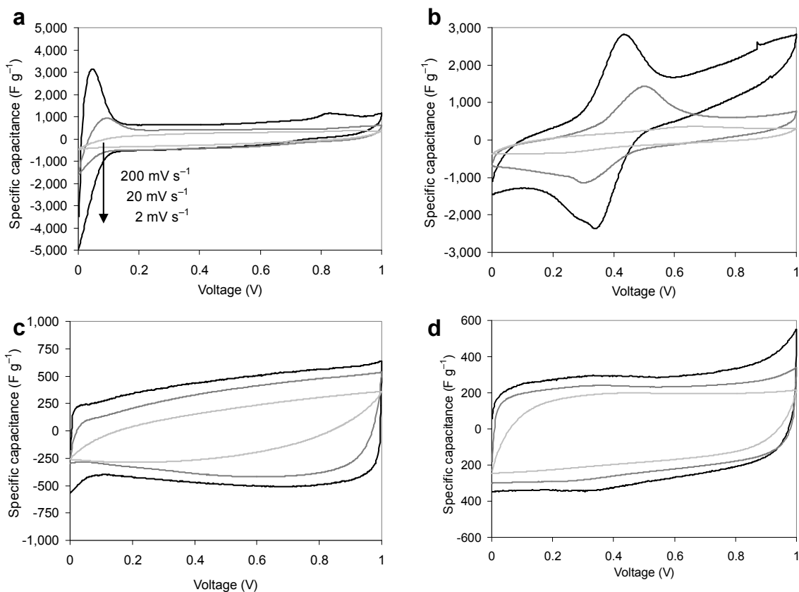
Figure 3-2 Cyclic voltammetry charts for SFC-9-800 in redox-active electrolytes at the sweep rate of 2, 20 and 200 \text{mV s}^{-1} .
