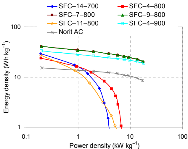
Figure 2-18 Ragone plots for the Cs salt-flux carbons in H 2 SO 4 .
