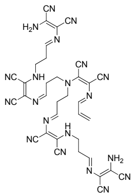
Figure 1–3 An oligomerized form example of acrodam. [38]
