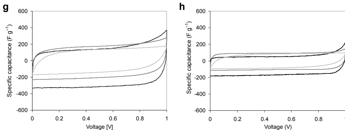
Figure 2–15 Cyclic voltammetry charts for the Cs salt-flux carbons in \text{H}_2\text{SO}_4 at the sweep rate of 2, 20 and 200 \text{ mV s}^{-1} (continued).
