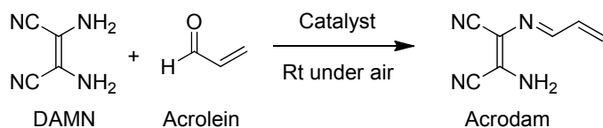
Scheme 1–1 Synthesis for acrodam.
