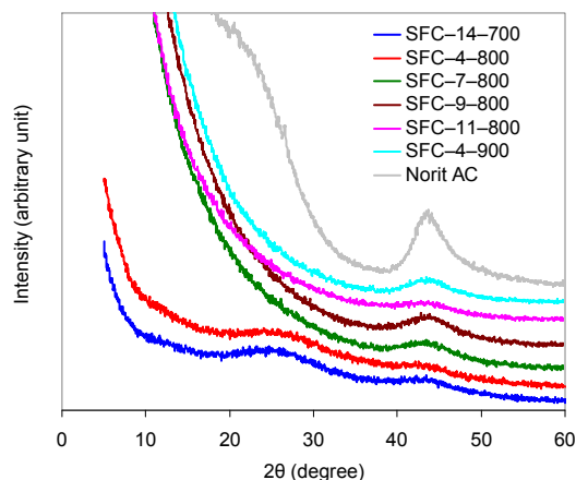
Figure 2–13 Wide angle X-ray scattering (WAXS) patterns for the Cs salt-flux carbons.
