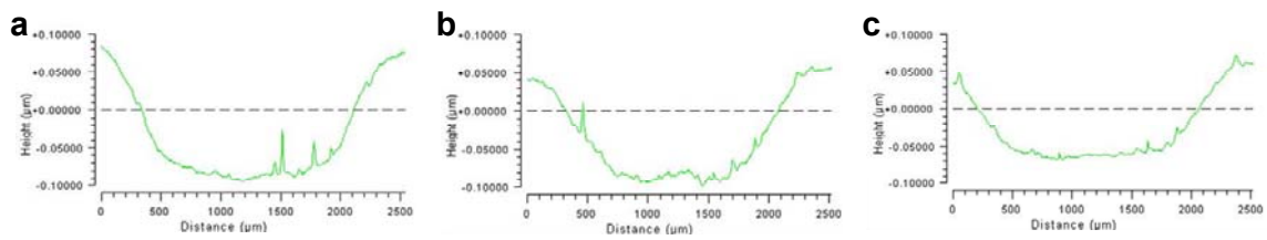
Figure 4–9 Topography measurements for the 10 min etched films using an optical surface profiler.
