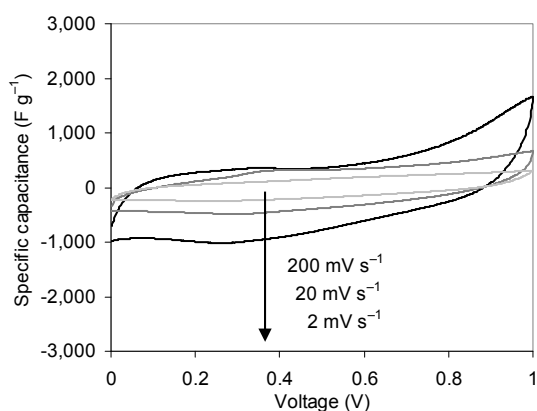
Figure 3–5 Cyclic voltammetry charts for SFC–9–800 in 0.5 \text{ mol L}^{-1} copper (II) sulphate dissolved in 1 \text{ mol L}^{-1} \text{ H}_2\text{SO}_4 aqueous solution ( \text{Cu}/\text{H}_2\text{SO}_4 ) as electrolyte at the sweep rate of 2, 20 and 200 \text{ mV s}^{-1} .
