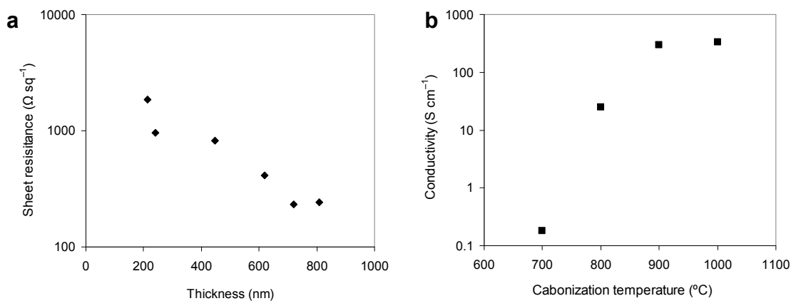
Figure 4–12 Electrical properties for the films.
