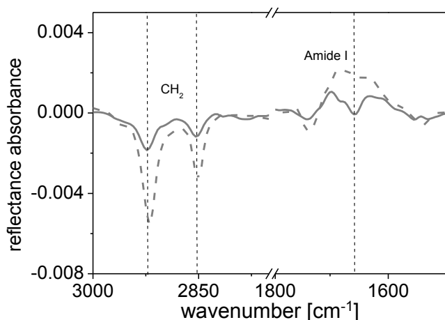
Figure 33: IRRA spectra of mixed films of DPPC/SM/LL-20 at \pi_{\text{eq}} = 10 mN/m (—) and \pi_1 = 25 mN/m (- - -) (5 mM HEPES, 100 mM NaCl, pH 7.4, 20°C, 0.2 \mu M peptide in solution).
