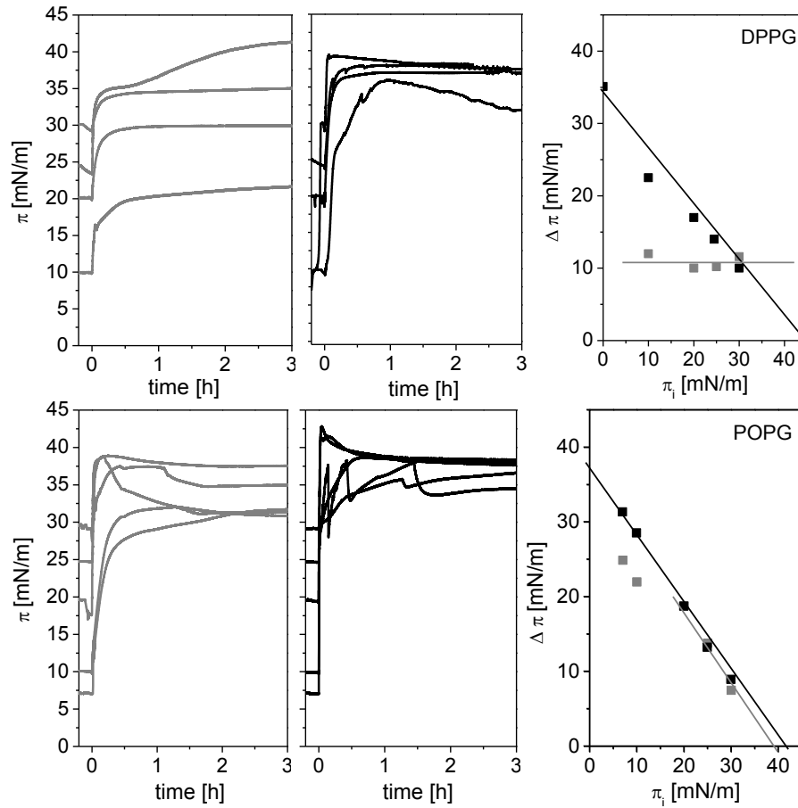
Figure 14: Estimation of the MIP of LL-20 (—, ■) and LL-32 (---, ■) into negatively charged DPPG and POPG monolayers. Shown is the time-depending surface pressure \pi for varied \pi_i . The increase in the surface pressure \Delta\pi dependent on the initial pressure \pi_i is plotted on the right. Extrapolating the linear fit to \Delta\pi = 0 gives the MIP. (5 mM HEPES, 100 mM NaCl, pH 7.4, 20°C, 0.2 \mu M peptide in solution).
