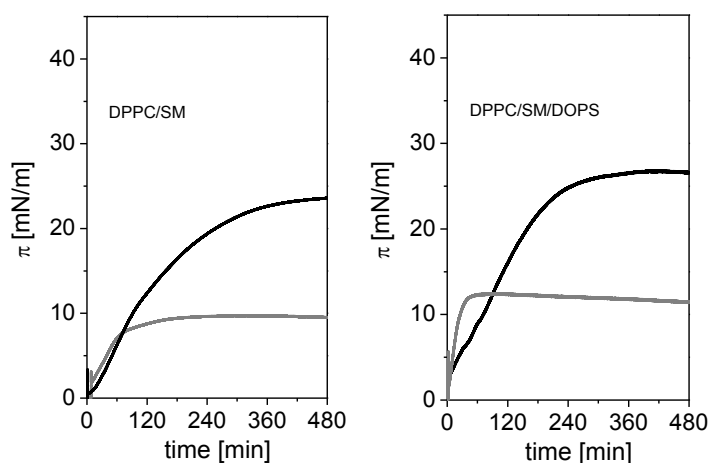
Figure 31: Time-dependent change in the surface pressure \pi upon adsorption of LL-32 (—) and LL-20 (---) to DPPC/SM (50:50) and DPPC/SM/DOPS monolayers (45:45:10). (5 mM HEPES, 100 mM NaCl, pH 7.4, 20°C, 0.2 \mu M peptide in solution).
