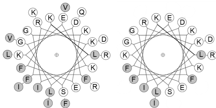
Figure 5: Helical wheel projection of LL-32 (left) and LL-20 (right). To emphasize the amphipathic structure of the peptides, hydrophobic amino acids are colored in grey (Eisenberg scale [146]).
