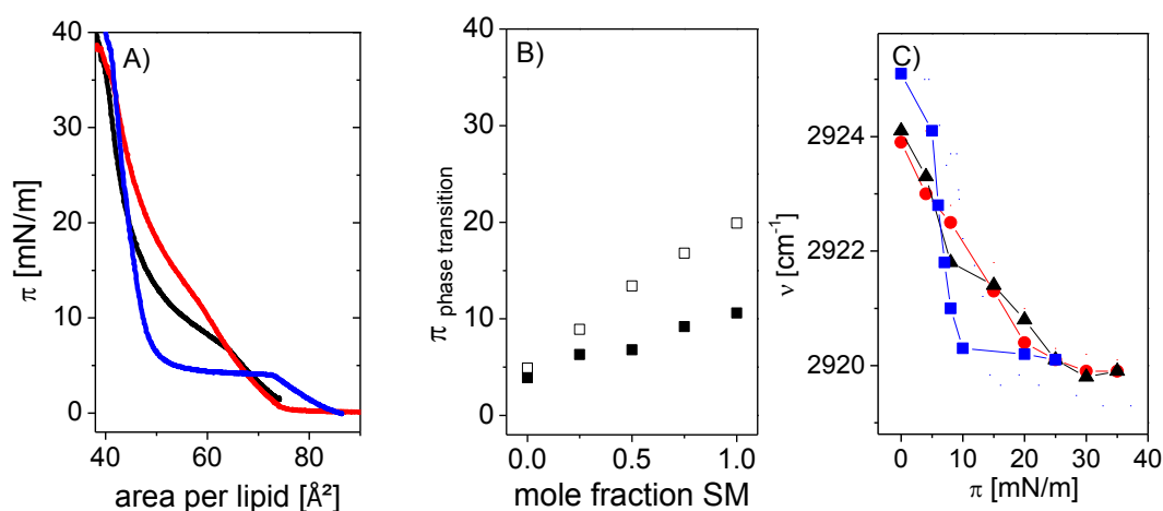
Figure 27: A) Isotherms and B) onset (■) and extrapolated end surface pressure (□) of the coexistence region for DPPC monolayers containing different mole fractions of SM. See text for description. C) Maximum in the asymmetric \text{CH}_2 vibration, depending on the surface pressure \pi . DPPC (—), DPPC/SM (50:50) (—) and SM (—). (5 mM HEPES, 100 mM NaCl, pH 7.4, 20°C)
