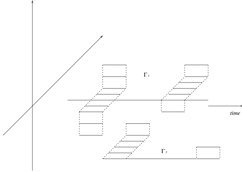
Figure 1: Two non-intersecting aggregates \Gamma_1 and \Gamma_2
