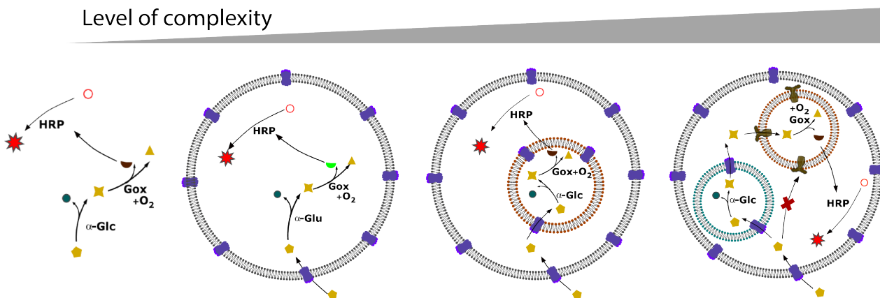
Figure 4.15: Schematic representation of the increasing levels of complexity from the bulk system to one-, two- and three- compartment systems.
