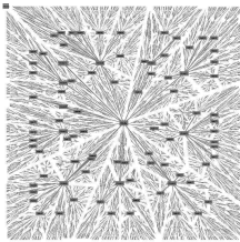
Space-optimized Tree
