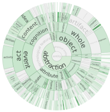
Sunburst View
