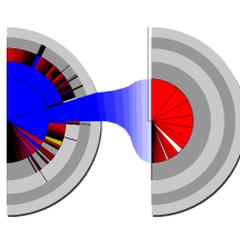
Information Slices
