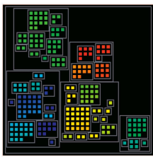
Data-Jewelry Box
