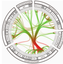
Bundle View
