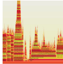
Flame Graphs
