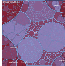
Voronoi Treemap
