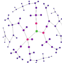
Tree Drawings
