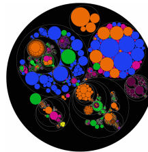
Pebbles Treemap
