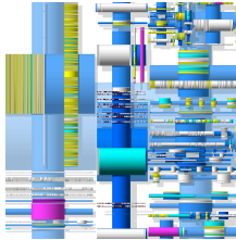
BeamTree
