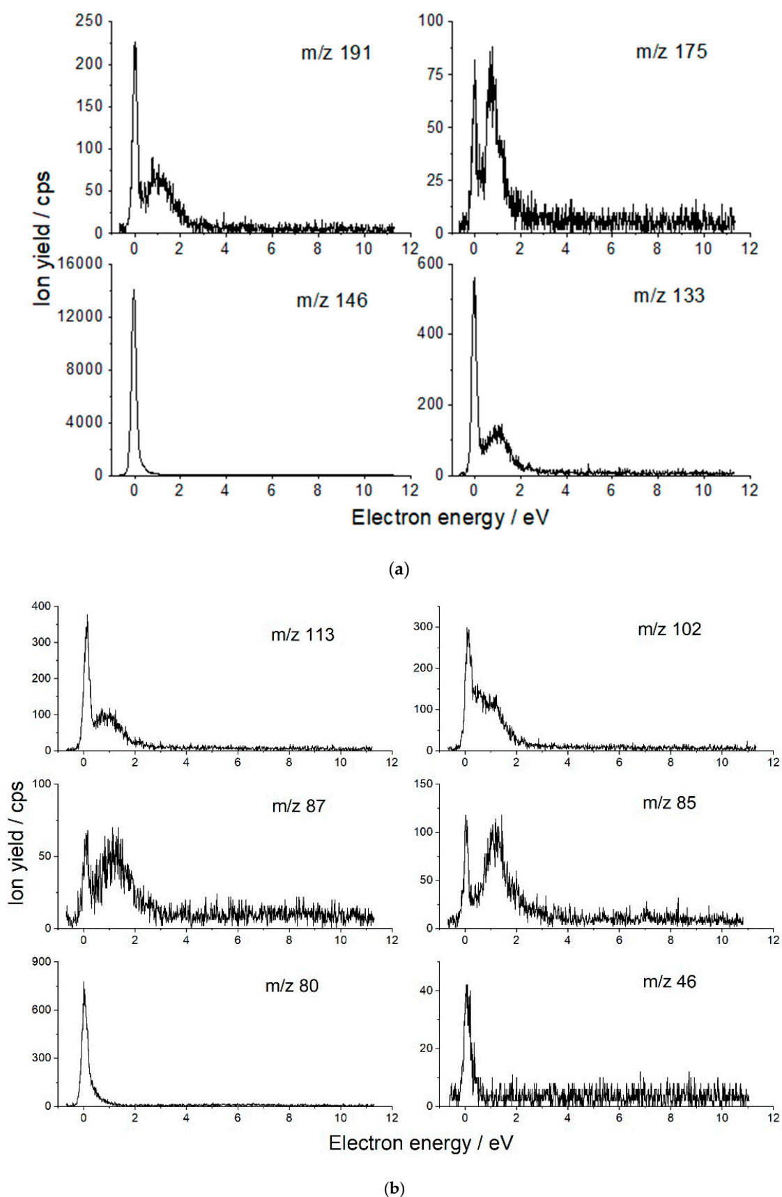
Figure 3. Anion yield functions of the citric acid: (a) fragment anions with m/z 191, 175, 146, and 133; (b) fragment anions with m/z 113, 102, 87, 85, 80 and 46.
