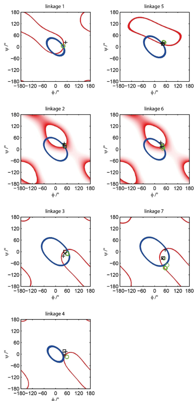
Figure 4. Distance curves for the octasaccharide describing the loci in terms of the glycosidic torsional angles \phi and \psi obtained by 2D ^1\text{H},^1\text{H} transfer NOESY NMR spectroscopy. Two-dimensional \phi, \psi distance-plots are shown for all glycosidic linkages, denoted by superscripts in the S. flexneri O-serogroup Y octasaccharide with the structure \alpha -L-Rhap-(1 \rightarrow 3) (1) - \beta -D-GlcpNAc-(1 \rightarrow 2) (2) - \alpha -L-Rhap-(1 \rightarrow 2) (3) - \alpha -L-Rhap-(1 \rightarrow 3) (4) - \alpha -L-Rhap-(1 \rightarrow 3) (5) - \beta -D-GlcpNAc-(1 \rightarrow 2) (6) - \alpha -L-Rhap-(1 \rightarrow 2) (7) - \alpha -L-Rhap. Conformational range calculated from methine trNOEs (blue lines) and methyl trNOEs (red lines) is shown, as determined from the effective proton-proton distances r_{ij} presented in Table S2. Overlaid are conformations obtained from six non-redundant X-ray models (green circles) or MD simulations of Sf6TSPwt with AMBER/Glycam06 (+, black pluses) or CHARMM ( \square , black squares) force fields. In addition, conformers calculated from MD simulations with the Sf6TSP E366A D399A are shown ( \times , black crosses, AMBER/Glycam06). These data points were obtained from Kang et al. [7] For the panels of linkages (2) and (6) the red colour gradient corresponds to the sum of the overlapped NOE cross-peak volumes of the NAG2-acetyl to RAM3-H4 and NAG6-acetyl to RAM7-H4. Red depicts the total volume of the overlapped signals and white corresponds to NOE being absent or stronger than the sum of the overlapped cross-peak volumes (Table S2).
