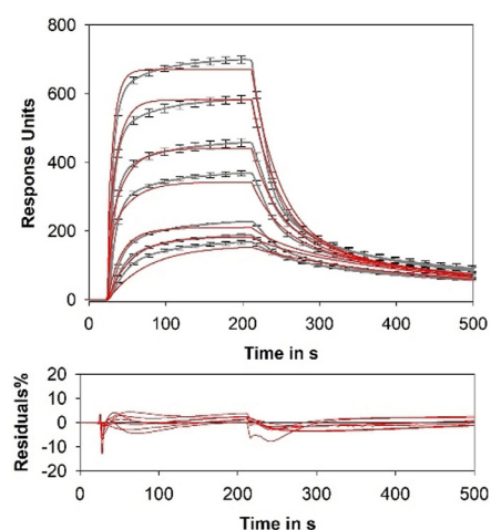
Figure 5. Surface plasmon resonance analysis of Sf6TSP binding to S. flexneri O-polysaccharide Y. SPR response curves obtained by injections of serial dilutions of Sf6TSP EADA (0.08–8 \mu\text{M} subunit concentration, grey, average of triplicate measurements with standard deviations shown for every 10th data point). Curves were fitted with a 1:2 heterogeneous binding model (red).
