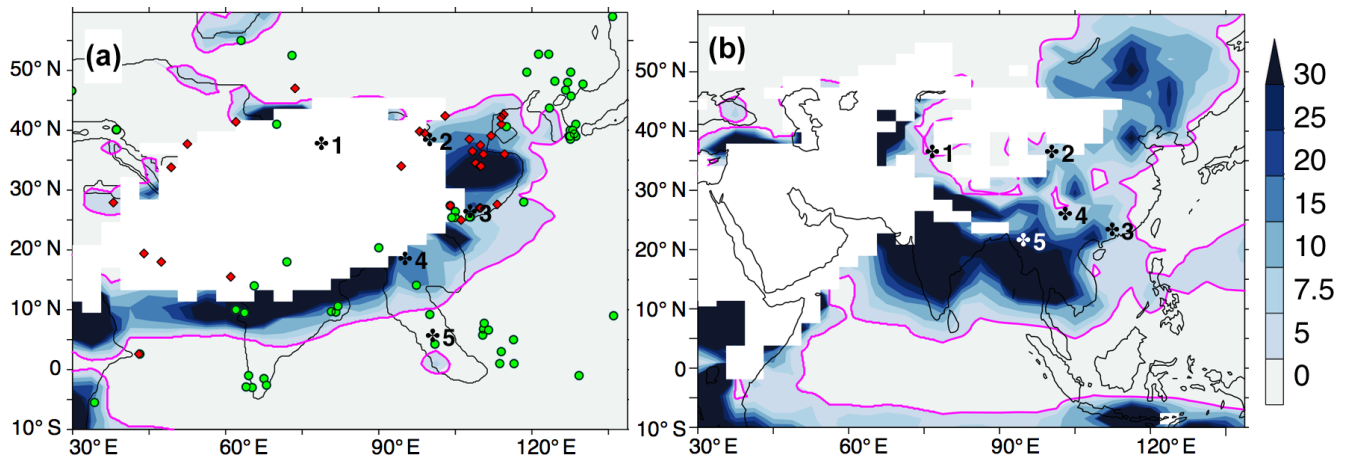
Figure 10. The 3W / 3D ratio for the (a) EOC4X and (b) control simulations. Regions receiving less than 1 \text{ mm d}^{-1} are kept blank. Overlaid magenta outline corresponds to the value 3W / 3D = 5 , considered as minimum value in modern monsoonal regions. We also highlight evaporite (red diamonds) and coal deposits (green circles) from Boucot et al. (2013), as well as the five highlighted regions described in the text.
