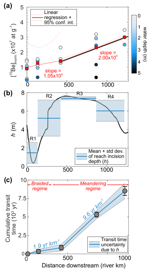
Figure 4. (a) ^{10}\text{Be}_{\text{norm}} and ^{10}\text{Be}_{\text{norm-DI}} (atoms \text{g}^{-1} ), calculated using Equation 3, plotted against distance downstream. Circles represent individual samples, colored by depth below the water surface. Error bars on individual sample points represent the propagation of analytical uncertainty and weighted error. Red squares show the depth-integrated, normalized concentrations with error bars representing the root-mean-square errors of Equation 1, normalized by ^{10}\text{Be}_{\text{reac}} . The red trend lines are linear regressions with 95% confidence interval fitted to the ^{10}\text{Be}_{\text{norm-DI}} data for the braided and meandering reaches, respectively. (b) Remobilization depth, h , measured along the channel (heavy black line) and mean remobilization depths for reaches 1–4 (R1–R4). (c) Cumulative transit time for each reach (heavy blue line) plotted against distance downstream, with minimum and maximum bounds associated with the standard deviation of h in each reach.
