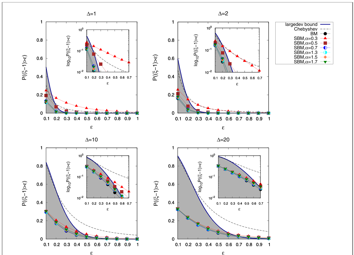
Figure H5. Variation of the estimates of P((\xi - 1) > \epsilon) with respect to \epsilon , for simulated SBM datasets of different anomalous diffusion exponent, with N = 300 , M = 10\,000 and different values of \Delta . Subdiffusive SBM with small values of the anomalous diffusion exponent \alpha fall out of the Brownian domain (grey-shaded region in the plot) for large values of the deviation parameter \epsilon , significantly at short lag times \Delta . This is in agreement with the behaviour of the EB parameter reported for SBM in [108], namely that for subdiffusive SBM the EB parameter (or equivalently the variance of the TAMSD) is larger for smaller values of the anomalous diffusion exponent. Moreover, for subdiffusive SBM, it was also reported in [108] that the EB parameter is larger for short lag times at fixed values of the anomalous diffusion exponent. This explains why subdiffusive SBM can be better distinguished from BM at small values of the lag time.
