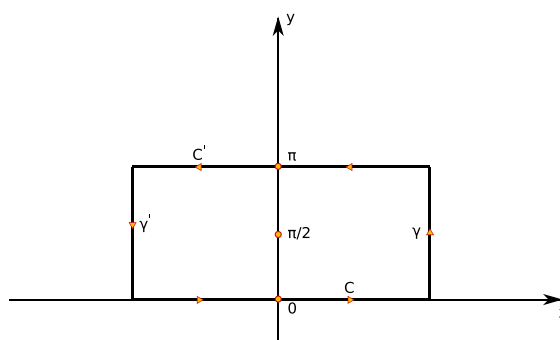
Figure D1. Contour of integration in equation (30).
