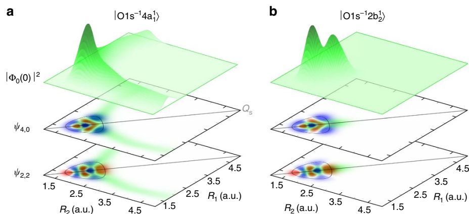
Figure 3 | Overlap between the core-excited and ground state wave functions. The squared integral wave packet |\Phi_0(0)|^2 (from Fig. 1d) versus R_1 and R_2 for the (a) |O1s^{-1}4a_1^> and (b) |O1s^{-1}2b_2^> core-excited states plotted against the vibrational wave functions \psi_{4,0} and \psi_{2,2} of higher delocalized states. Isoenergetic curves for the (4, 0) and (2, 2) vibrational states are shown with thin lines. The crossing Q_s line represents the symmetric stretching coordinate.
