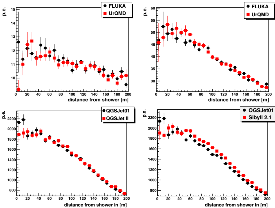
Fig. 15 Comparison of the Cherenkov light profiles for proton-induced showers generated with different hadronic interaction models. The profiles for FLUKA and UrQMD at 50 GeV ( left ) and 100 GeV ( right ) are shown in the top panel. Two QGSJet versions and SIBYLL at 1 TeV are compared in the bottom panels
