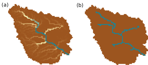
Figure 5. Illustration of the stream network used in this study. (a) Original stream network based on the streamflow routing algorithm of mHM; (b) processed stream network that was used in this study. The small tributaries where the runoff rates are below the threshold ( 0.145 \text{ m}^3 \text{ s}^{-1} ) as shown in panel (a) have been removed to form panel (b).
