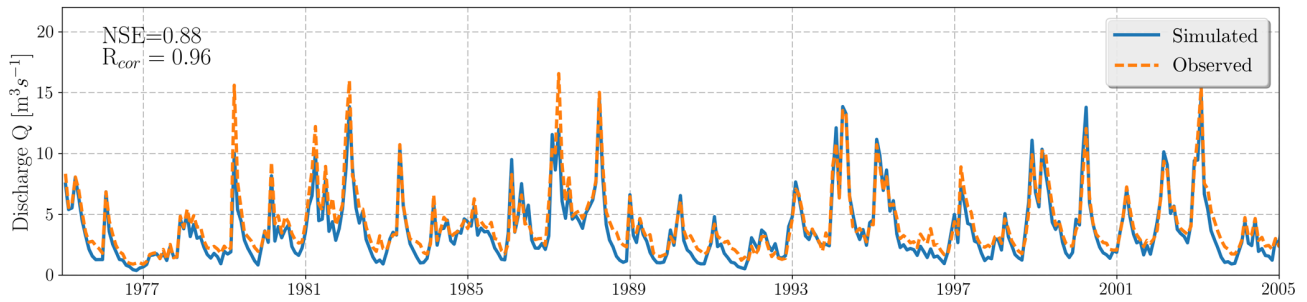
Figure 6. Observed and simulated monthly discharge at the outlet of the Nagelstedt catchment.
