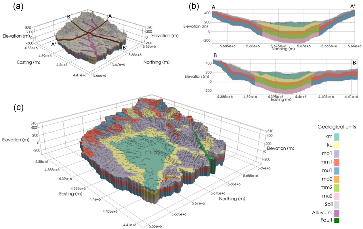
Figure 4. Three-dimensional and cross-sectional views of the hydrogeologic zonation in the Nängelstedt catchment. Panel (a) highlights the distribution of alluvium and soil zones. Panel (b) shows two vertical geological cross sections. Panel (c) shows the detailed zonation of geological sub-units beneath the soil zone and alluvium.
