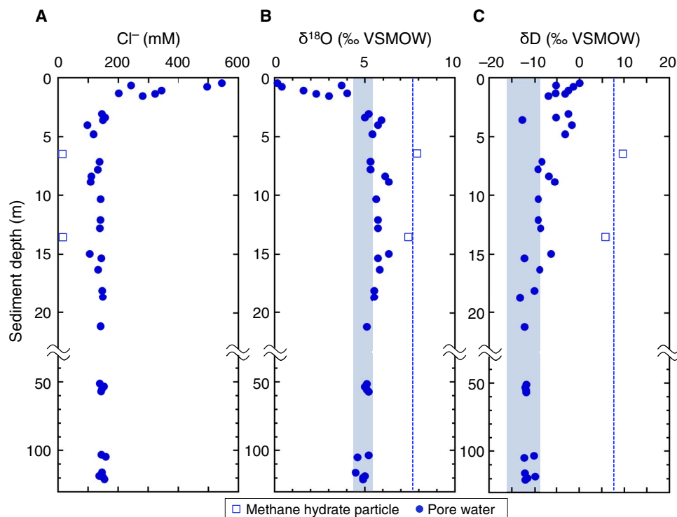
Fig. 2. Chloride concentration and stable isotopic compositions of pore water in sediments of KMV#5. Vertical profile of Cl - (A), \delta^{18}\text{O} (B), and \delta\text{D} (C) of pore water in sediments. Circle and square plots represent pore water sample and water from dissociated gas hydrate fragment, respectively. Dashed line represents the averaged isotopic value of methane hydrates, and blue-filled range denotes original \delta^{18}\text{O} and \delta\text{D} values of pore water before the formation of methane hydrates.
