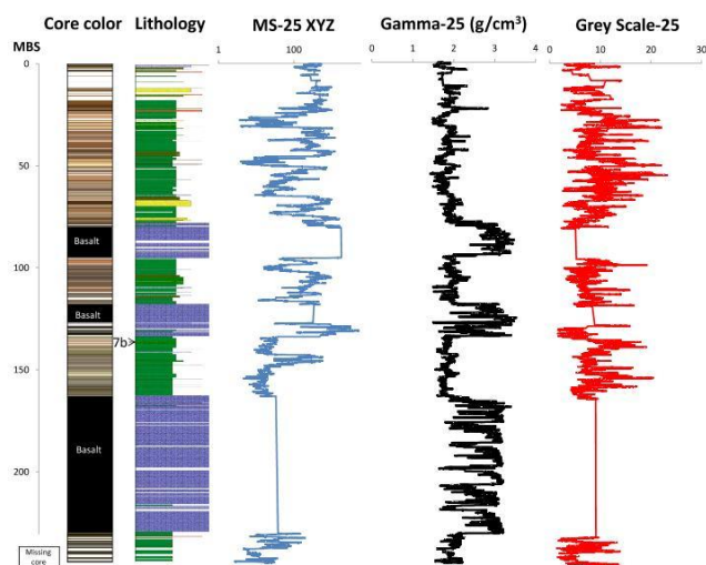
Figure 6. Summary stratigraphy of core HSPDP-NAW14-1A, from the Woranso locality, Northern Awash drilling area, northern Ethiopia, based on initial core description results. Columns from left to right: core color stratigraphy; lithologic log; see Fig. 5 for the key to lithologies used in all cores illustrated; composite of magnetic susceptibility (MS) log data (25-point running mean smooth) from LacCore Geotek ® XYZ point sensor data; composite of induced gamma density log data (25-point running mean smooth, spurious values < 1.4 \text{ gm cm}^{-3} removed); composite of spectrophotometric grey-scale log data (25-point running mean smooth). All data collection, instrumentation, and parameters as in Fig. 5.
