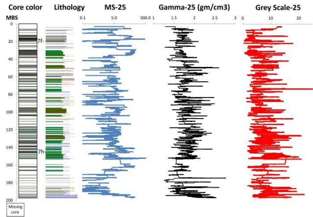
Figure 13. Summary stratigraphy of core HSPDP-MAG14-2A, from the Lake Magadi drilling area, southern Kenyan Rift Valley, based on initial core description results. Columns from left to right: core color stratigraphy; lithologic log; see Fig. 5 for the key to lithologies used in all cores illustrated; composite of magnetic susceptibility (MS) log data (25-point running mean smooth) from LacCore Geotek ® XYZ point sensor data; composite of induced gamma density log data (25-point running mean smooth, spurious values < 1.2 gm cm -3 removed); composite of spectrophotometric grey-scale log data (25-point running mean smooth). All data collection, instrumentation, and parameters as in Fig. 5.
