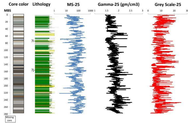
Figure 14. Summary stratigraphy of core HSPDP-CHB14-2A, from the Chew Bahir drilling area, southern Ethiopian Rift Valley, based on Initial Core Description results. Note: coring gaps in CHB14-2A are almost entirely infilled by matching to the twinned borehole CHB14-2B (not illustrated), collected immediately adjacent to this core. Columns from left to right: Core color stratigraphy; lithologic log; see Fig. 5 for the key to lithologies used in all cores illustrated; composite of magnetic susceptibility (MS) log data (25-point running mean smooth) from LacCore Geotek ® XYZ point sensor data; composite of induced gamma density log data (25-point running mean smooth, spurious values < 1.4 gm cm -3 removed); composite of spectrophotometric grey-scale log data (25-point running mean smooth). All data collection, instrumentation, and parameters as in Fig. 5.
