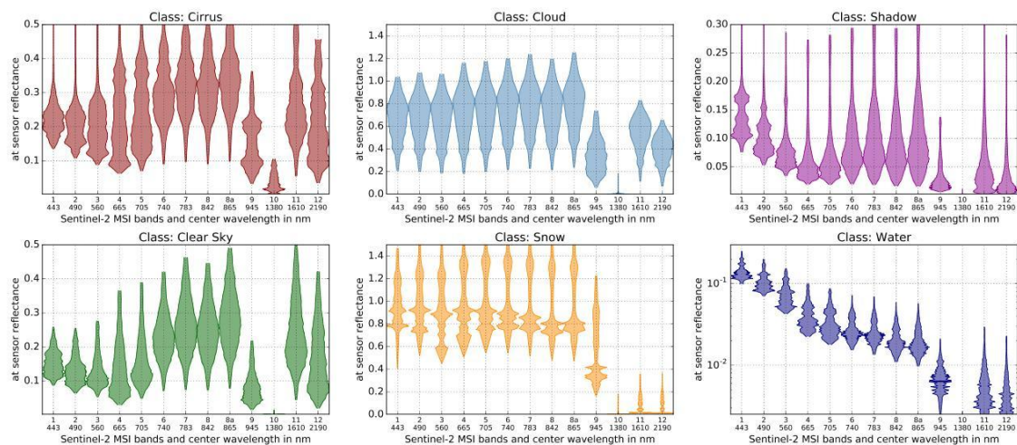
Figure 1. Spectral histograms of the database per class and Sentinel-2 MSI channel. Each panel shows histograms for a single classification class and the data is presented as a Violin plot, where each histogram is normalized to its maximum and is vertically shown on both sides of the baseline line for each channel.
