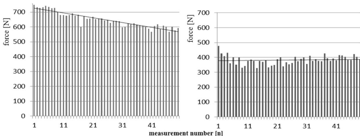
Fig 5. Values of AF_{ecc\_max} of two subjects during 50 repetitions with a linear trend line. (left: R^2=0.868 ; right: R^2=0.012 ).
