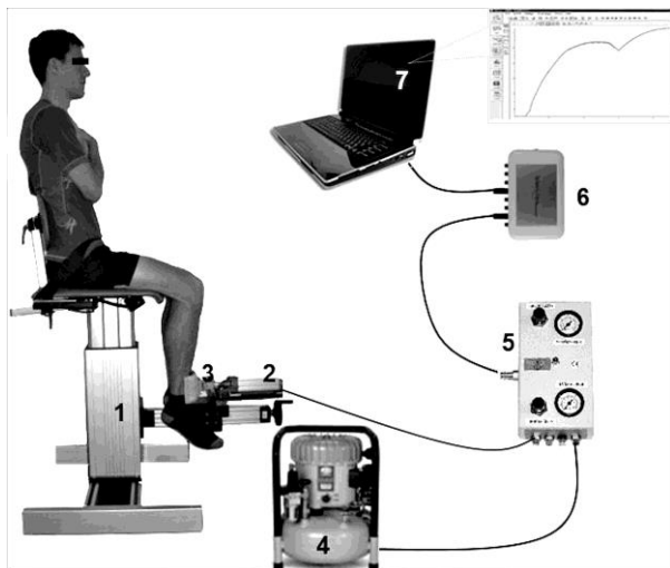
Fig. 1 Measuring system to determine the Adaptive Force
