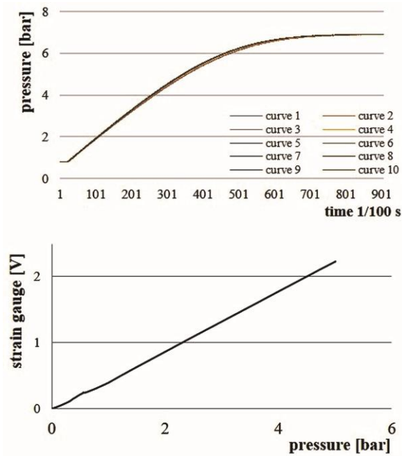
Fig 4. Above: Diagram of ten pressure curves measured in a row (sampling rate 100 Hz). Below: Scatter diagram between rises of the strain gauge and of the pressure signal.
