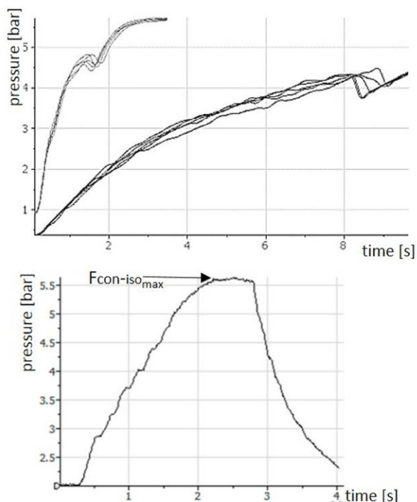
Fig. 3. Pressure curves [bar] measured by the system SeBit knee. Above: Five trials of measuring the AF of one subject during slow (black) and rapid (grey) pressure increase. The data are filtered with butterworth filter (filter degree 10, cut-off frequency 3 Hz). Bottom: One trial of maximum concentric-isometric force F_{con-iso_{max}} .
