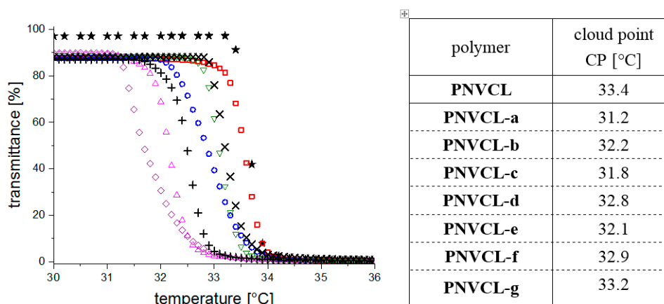
Figure 4. Temperature dependent turbidimetric analysis of PNVCL and dye-labeled NVCL copolymers in aqueous solutions (3.00 g·L -1 , heating rate 0.2 K·min -1 ). (★) = PNVCL , (◇) = PNVCL-a , (○) = PNVCL-b , (△) = PNVCL-c , (▽) = PNVCL-d , (+) = PNVCL-e , (×) = PNVCL-f , (□) = PNVCL-g . The phase transition temperatures were taken as the temperature of the onset of clouding (cloud points CP).
