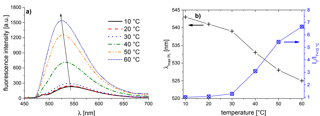
Figure 10. Temperature dependent fluorescence behavior of PNVC-L-f in aqueous solution (concentration 0.10 \text{ g} \cdot \text{L}^{-1} ): (a) normalized emission spectra ( \lambda^{\text{Exc}} = 418 \text{ nm} ); and (b) evolution of \lambda_{\max}^{\text{Em}} of the emission band, and of the fluorescence intensity normalized to 10^\circ\text{C} .
