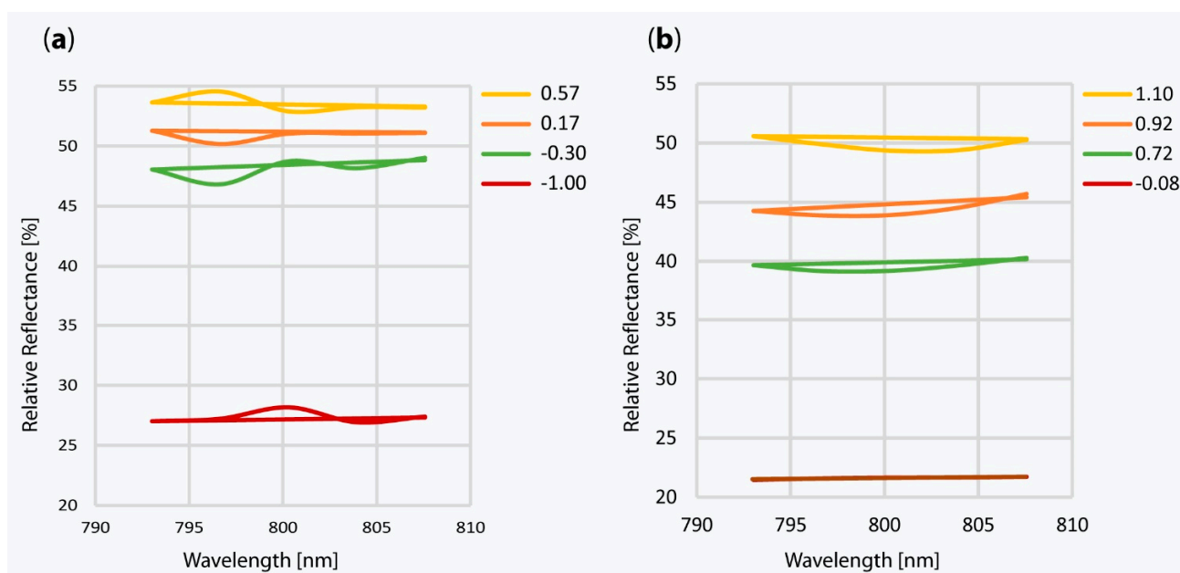
Figure 8. A comparison between four image spectra with and without applying R-L deconvolution. (a) Image spectra from the simple run (without R-L deconvolution); and (b) image spectra from the full approach (including R-L deconvolution). The legend values represent the absorption depth (difference between the absorption band at 803 nm and its corresponding value in the continuum). Deconvolution has a high potential for mapping the exact borders of these zones, especially for transition pixels at the outer zones of the REE-enriched parts. Modified after Boesche et al. 2014 [23].
