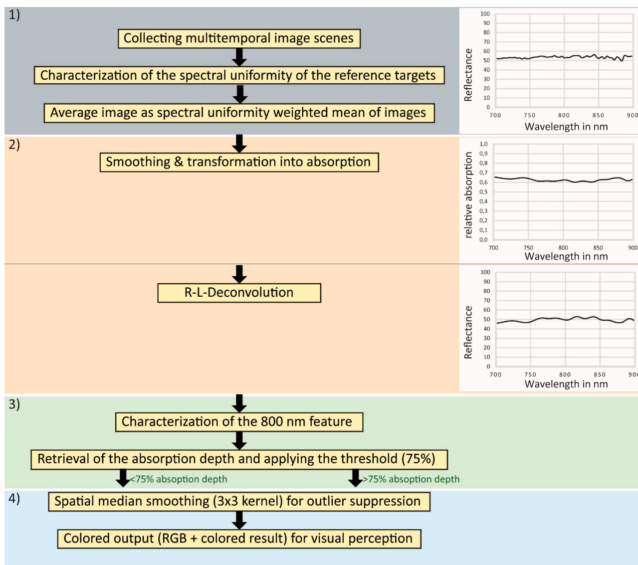
Figure 4. Flow Chart of the REE mapping approach showing the four main steps of its application. The first step is the collection of the multitemporal data cube and preprocessing. The second step is the application of Richardson-Lucy deconvolution. The third step is the identification and characterization of indicative and discriminative absorption bands and image pixel clustering. The fourth step describes the post-processing of the data and visualization.
