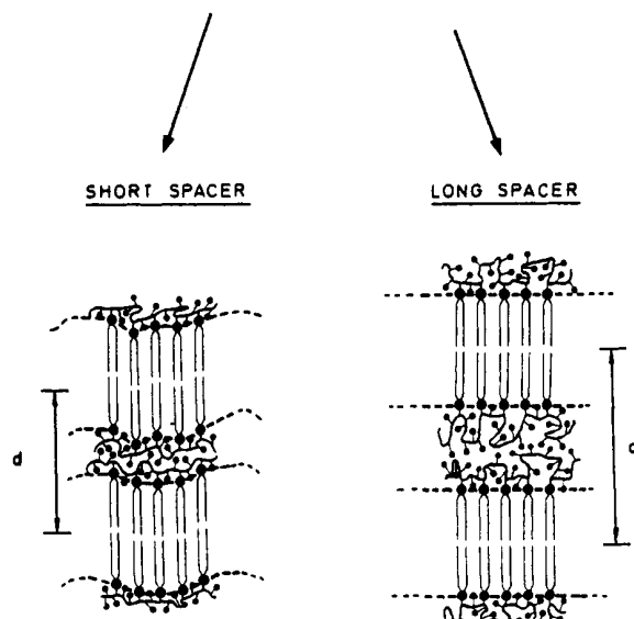
Figure 7. Schematic representation of the layer thickness ( d ) and layer correlation (---) in dependence of the length of the main chain spacer (short spacer: m = 1.2 ; long spacer: m = 8.5 ).
