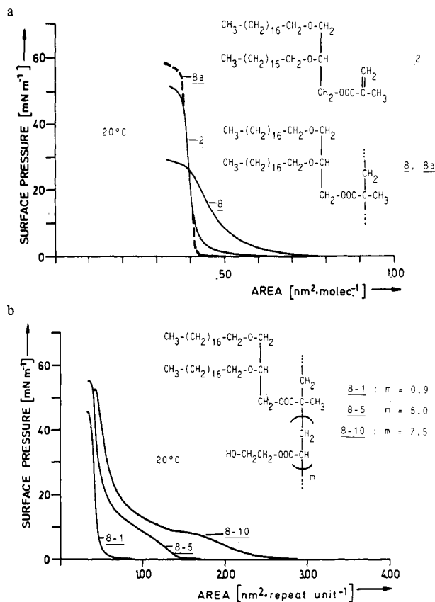
Figure 1. Isotherms of monomer 2 , homopolymer 8 (prepolymerized in solution before spreading) and homopolymer 8a (polymerized in monolayer after spreading) on water at 20 °C. (b) Isotherms of the amphiphilic copolymers 8-1 , 8-5 , and 8-10 on water at 20 °C.
