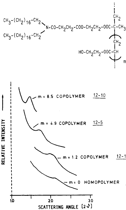
Figure 5. X-ray scattering diagrams prepared from polymeric amphiphiles ( 12 to 12-10 ) with various comonomer contents.
