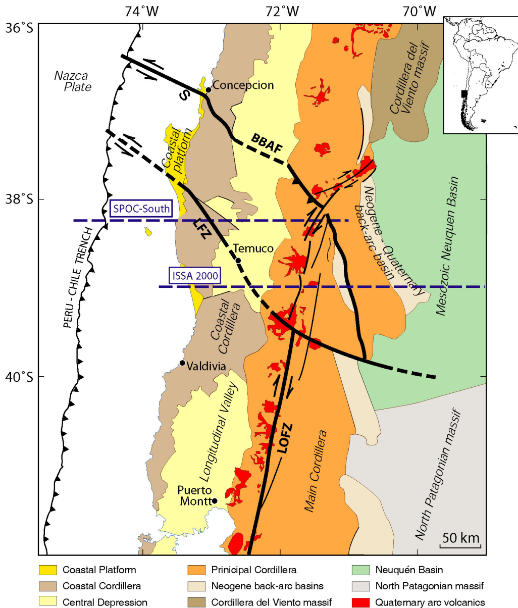
Figure 3.2: Geological map of the southern Chilean segment (36° - 42°S) showing major morphostructural units and fault zones. LOFZ - Lofquín-Ofqui Fault Zone, LFZ – Lanahue Fault Zone, BBAF – Bio-Bio-Aluminé Fault. Dashed lines indicate positions of the SPOC-South and ISSA 2000 seismic experiments. (after Melnick & Echtler, 2006)
