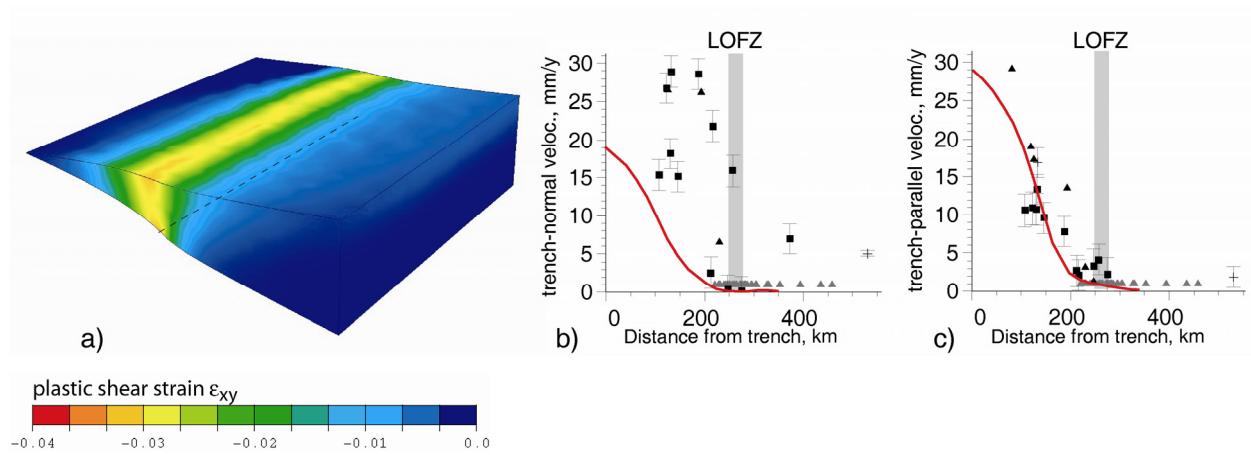
Figure 6.20: Preferential model for southern Chilean study area. (a) illustrates the plastic shear strain, \epsilon_{xy} , colour coded. (b) and (c) show the comparison of surface velocity distribution (trench-normal and trench-parallel) resulting from the model with GPS measurements (symbols, see section 3 for details of GPS data; LOFZ - Liquiñe-Ofqui Fault Zone).
