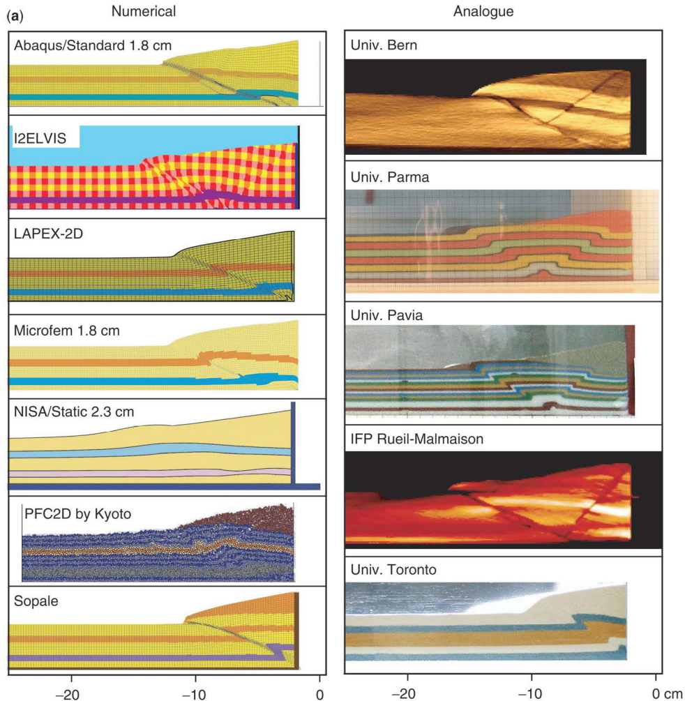
Fig. 6. Comparison of numerical and analogue results for the shortening experiment. (a) 2 cm of shortening (note that the model domain has been cropped on the left-hand side). (b) 14 cm of shortening. WebColor
