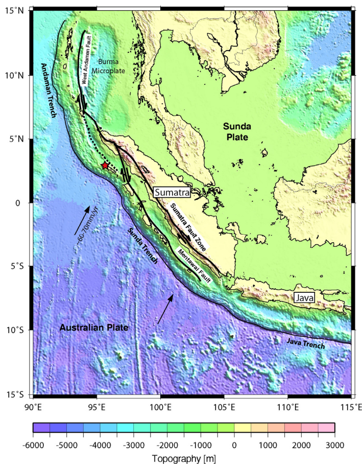
Figure A2.5: Topographic map of the Sumatra subduction zone; solid lines indicate the Sunda trench and the margin parallel strike slip faults; arrows show the convergence direction, red star indicates the epicenter of the 2004 Sumatra- Andaman earthquake.
