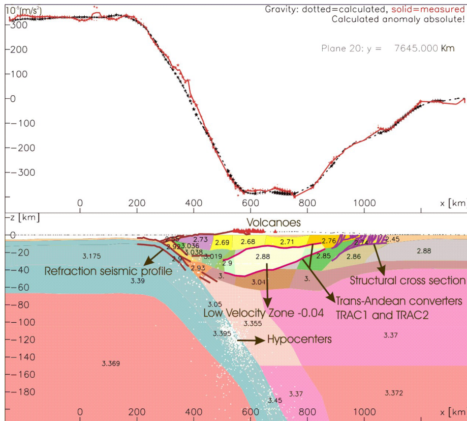
Figure 3.9: Model of Prezzi et al. (2005): density distribution along 21.3^\circ\text{S} (bottom panel) and comparison between calculated and measured Bouguer anomaly (upper panel). Good correlation between two lines on the upper panel indicates reliability of the resolved density structure.
