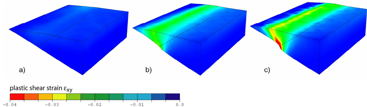
Figure 6.7: Comparison of deformation in models with different coefficient of basal friction, \mu_b : 0.2 (a), 0.4 (b, reference model), and 0.5 (c). The intensity of deformation clearly correlates with the value of basal friction.
