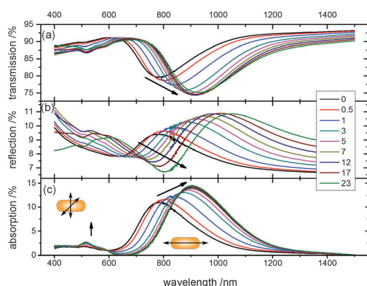
Fig. 6 Series of transmission (a), reflection (b), and calculated absorption (c) spectra for GNR type 1. The arrows indicate the spectral changes due to covering the particles with double-layers (DL) of PSS/PAH. The pictures in (c) illustrate the transverse plasmon absorption at \sim 520 nm and the longitudinal one in near infrared.
