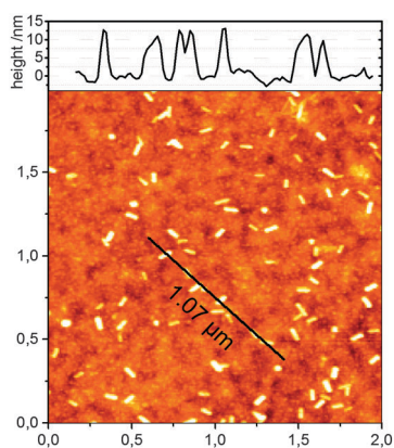
Fig. 3 AFM pictures of GNR type 1 on 2 \times 2 \mu\text{m}^2 . The upper panel shows the topographic cross section along the black line.
