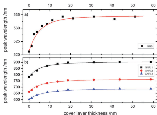
Fig. 8 The peak-shift calculated for 20 nm-GNSs (a, line) and for all three types of GNRs (b, lines) corresponds very well to the measured shifts (a and b, symbols). The calculation assumes an adjusted real-part of \epsilon_{\text{Au}} (Fig. 5) inferred from the measured values for fully polymer-embedded GNS and for GNS emerged in distilled water.
