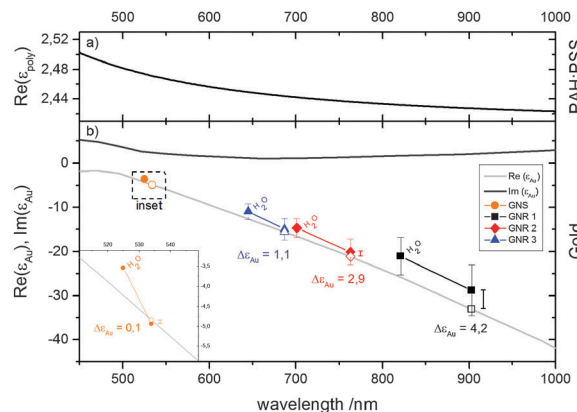
Fig. 5 Plot of the dielectric function of PSS/PAH multilayers, \epsilon_{\text{poly}} , (upper graph) and bulk-gold, \epsilon_{\text{Au,bulk}} , measured by Johnson and Christy 48 (lower graph, grey lines). The values for \epsilon_{\text{Au}} inferred from the LSP resonance wavelength and \epsilon_{\text{poly}} by MGEM (lines & closed symbols) considerably differ from \epsilon_{\text{Au,bulk}} (open symbols) for all types of particles. The symbols marked with \text{H}_2\text{O} correspond to measurements of particles dispersed in distilled water. Error bars illustrate the uncertainties introduced by the measured size of the GNR via the shape factor G_A .
