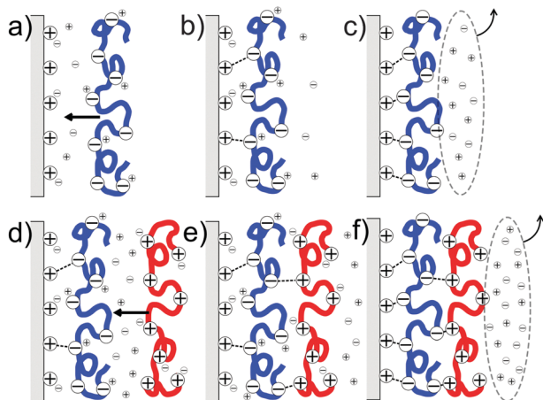
Scheme 1 Schematic illustration of layer-by-layer deposition. A negative charged polyelectrolyte (e.g. PSS) binds to a positive charged surface (a and b). Due to washing, the remaining counterions ( \text{Na}^+ , \text{Cl}^- ) are removed and additional bonds are formed (c). In ionic solution, some bonds break up (d) and a positive charged polyelectrolyte (e.g. PAH) can adsorb (e). After washing and reformation of bonds (f) the process can be continued with the first step.
