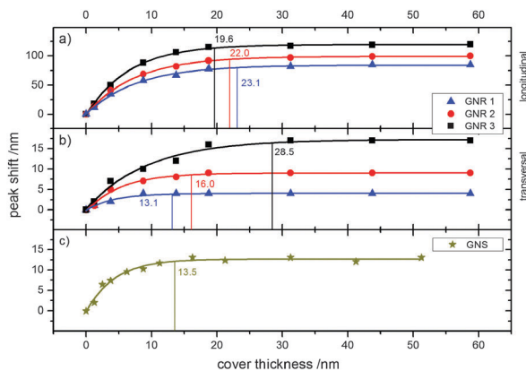
Fig. 7 Shift of plasmon resonance depending on cover layer thickness. The lines are polynomial fits according to (A - B/r^6) , where r is the cover layer thickness, A is the saturation asymptote and B is an arbitrary fitting parameter. The marked values of layer thickness correspond to 95% of saturation parameter A . The longitudinal LSPs (a) saturate for different values than the transverse LSP (b) of the GNRs. The LSP of the GNS (c) saturates at a similar value as the transverse LSP of the smallest GNR, which has a width comparable to the size of the GNS.
