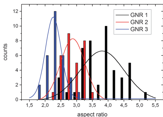
Fig. 2 Distribution of aspect-ratio of GNR extracted from the SEM images in Fig. 1. In particular GNR type 1 particles have a very broad size distribution.
