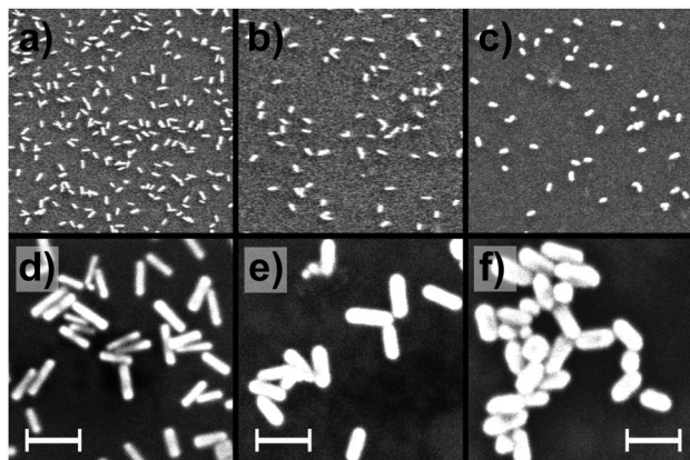
Fig. 1 SEM pictures of the used GNRs type 1 (a and d), 2 (b and e), and 3 (c and f). The upper panel shows the in-plane distribution of the spectroscopically analyzed samples on an area of 2 \times 2 \mu\text{m}^2 . Below are high resolution pictures on Si substrates for size determination given in Table 1. The white bars represent 100 nm.
