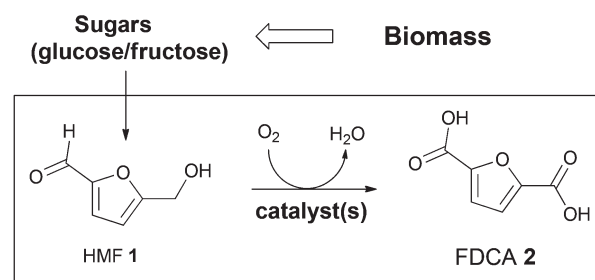
Scheme 1 Desired route to FDCA from biomass derived sugars.
