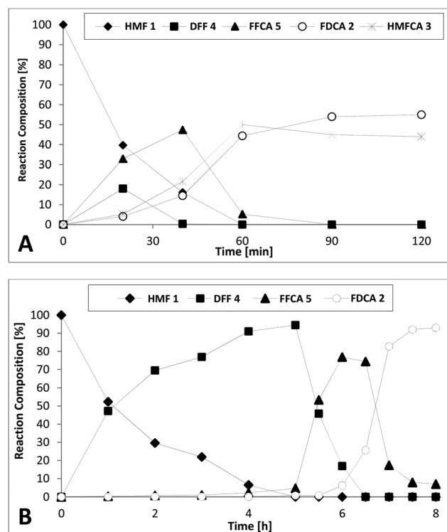
Fig. 1 Enzyme cascades for conversion of HMF ( 1 ) with (A) dual combined enzymes (GOase M 3–5 + PaoABC) ([HMF] = 20 mM) and (B) one-pot sequential reaction ([HMF] = 50 mM).
