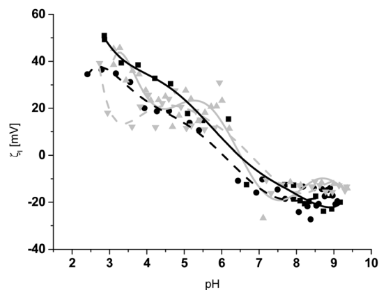
Fig. 3 \zeta_1 plot of hOG-OMe (▲: run pH 3 → 9; ▼: run pH 9 → 3) and hPG-OMe (■: run pH 3 → 9; ●: run pH 9 → 3). For hOG-OMe the plateau between pH 4 and 6 at positive \zeta_1 values suggest free amino groups, while the pronounced minimum of the curve at pH 7.5 indicates imide cleavage during the measurements, which can be interpreted by some parts of the PEI membrane surface being exposed during the measurements. In the case of hPG-OMe, which is representative also for the other hOG/hPG functionalized surfaces, mainly \text{OH}^- adsorption was observed, which suggests a complete surface coverage. The lines (grey hOG-OH, black: hPG-OH, compact pH 3 → 9, dashed pH 9 → 3) are added as guides to the eye.
