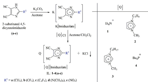
Scheme 1 Synthetic strategy of imidazolate-anion based ILs.
