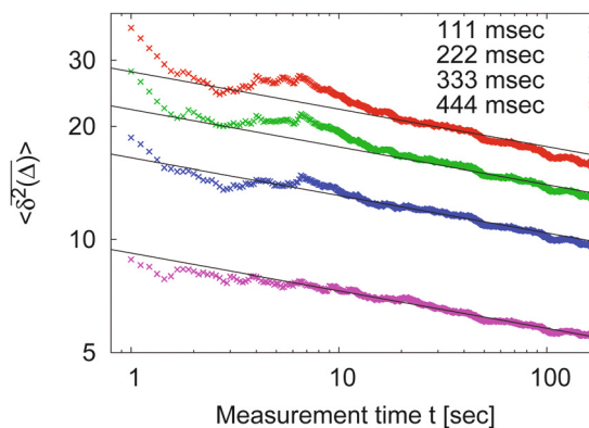
Fig. 7 Dependence of the time averaged MSD on the measurement time, observed for the motion of potassium channels in the plasma wall of human kidney cells in ref. 50. The straight lines show the scaling \overline{\delta^2} \simeq 1/t^{1-\alpha} with \alpha = 0.9 deduced from the statistics of waiting times of this system shown in Fig. 5. The predicted scaling is nicely fulfilled by the data, corroborating the ageing nature of the system: the longer the system evolves (given by the times in the figure key) the smaller the apparent diffusivity. Data courtesy Diego Krapf, Colorado State University.
