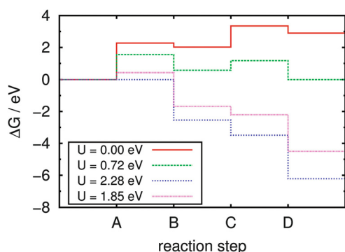
Fig. 10 Calculated free energy steps during the anodic water oxidation process at \text{pH} = 7 . Continuous red line: no external potential/irradiation; dashed green line: equilibrium situation; dotted blue line: “all downhill” limit; dotted pink line: irradiated sample. No qualitative changes are observed for different values of \text{pH} ; see text for a detailed discussion.
