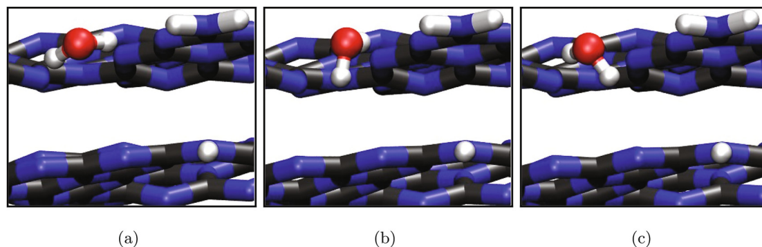
Fig. 8 Stable water adsorption geometries on the (\bar{1}010) surface (SCC-DFTB) as mentioned in the text.
