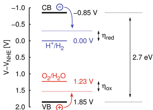
Fig. 1 Schematic illustration of band positions in g\text{-C}_3\text{N}_4 (at \text{pH} = 7 ) relative to the normal hydrogen electrode (NHE) as given in ref. 8. VB/CB: valence/conduction band; \eta_{\text{ox}}/\eta_{\text{red}} : overpotential for water oxidation/ \text{H}^+ reduction.
