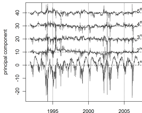
Figure 4.3: Scores of the first five principal components. Every component is shifted by +10 to improve visibility.
