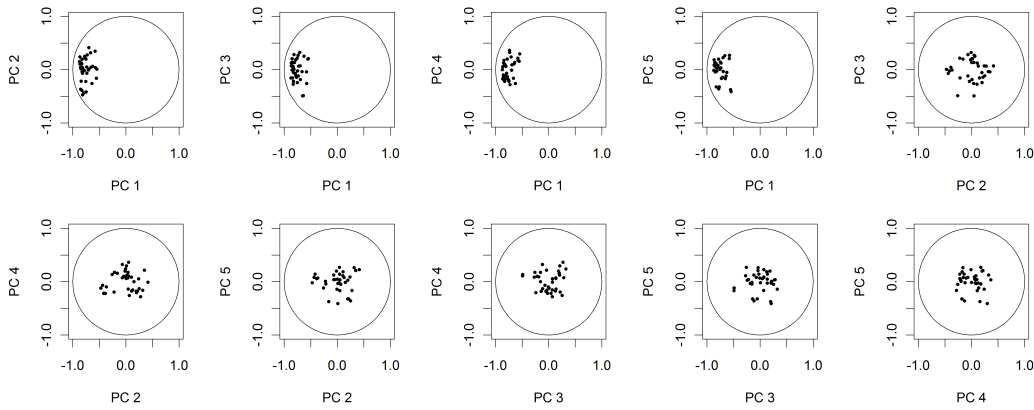
Figure 4.5: Biplots of loadings of the first five components compared to the unit circle.
