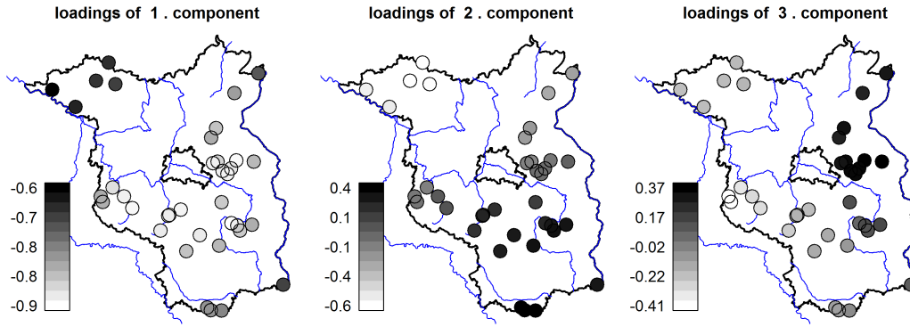
Figure 4.7: Loadings of the first three principal components of precipitation data (1991 to 2006).
