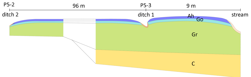
Figure 3.2: Geometry of the model domain and implemented soil layers. The soil body was divided into four different layers (Ah, Go, Gr and C) and three colmatation layers around the stream and ditches.
