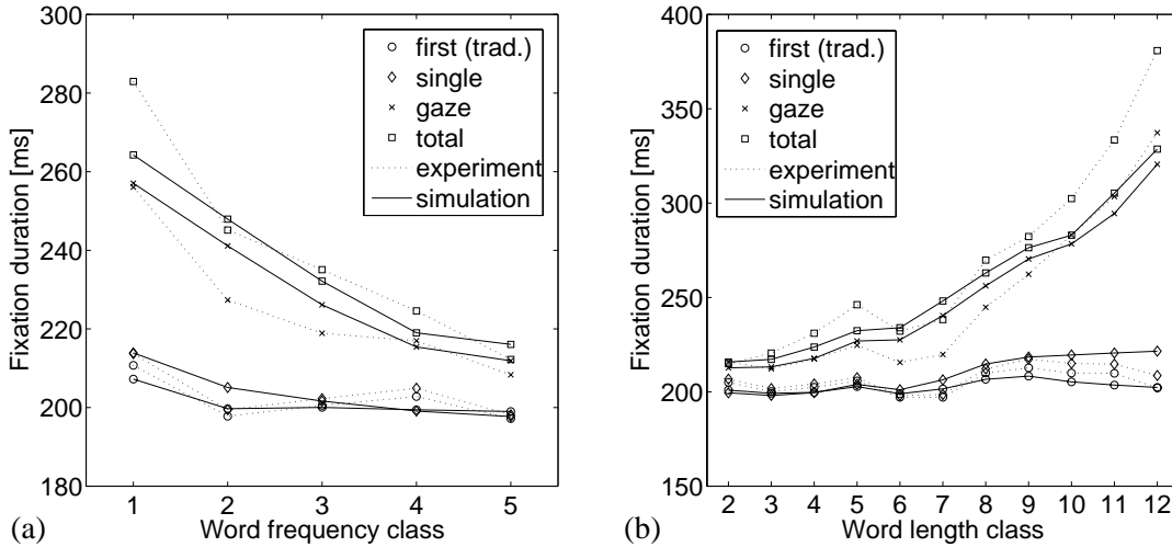
Figure 28: Results on gaze duration and traditionally defined first fixation duration. (a) Fixation duration as a function of word frequency class. (b) Fixation duration as a function of word length.
