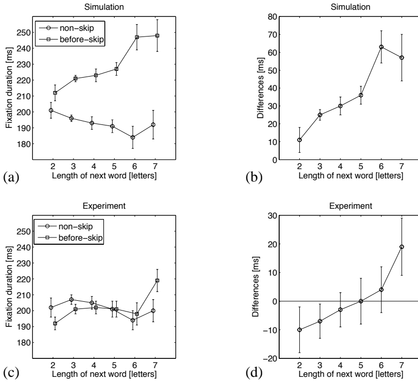
Figure 20: Analysis of costs for word skipping from statistical analysis. (a,b) Model simulations. (a) Fixation durations increase with word length (of the skipped word) before a skip and slightly decrease with word length before a non-skip. There are global costs. (b) The differences between cases of skips and non-skips increases approximately linearly with word length. (c,d) Experimental data. (c) There are reduced fixation durations before short skipped words and costs before longer skipped words compared to non-skipped cases. (d) The difference increases linearly with the length of the skipped word.
