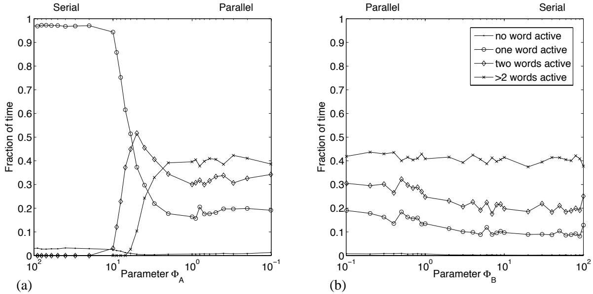
Figure 22: The transition from parallel to serial processing in the SWIFT model. (a) If the processing rate is controlled by parameter \phi for both preprocessing and lexical completion, then we observe a sharp transition to serial processing \Lambda_1 \approx 100\% for \phi \approx 10 . (b) When lexical completion is modulated by \phi with preprocessing fully parallel, the distribution of activation over words is even broader than in the SWIFT model.
