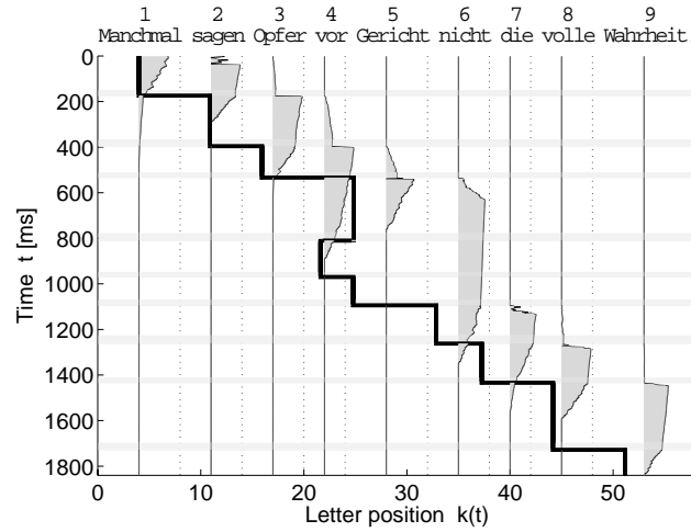
Figure 7: Example for the numerical simulation of the SWIFT model. Time evolves along the vertical axis. The fixation position k(t) is indicated by the black line in units of letters. Activations a_n(t) are given by the dark grey areas, while saccades are indicated by the horizontal line in light grey.
