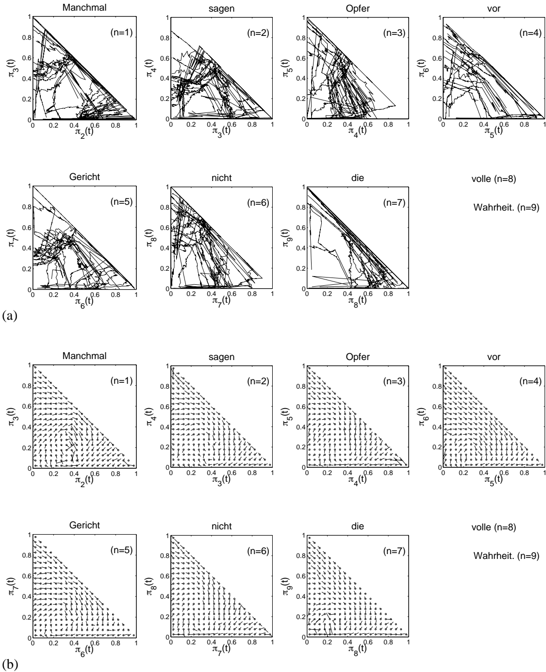
Figure 26: Visualization of SWIFT's temporal evolution in reduced phase space. (a) Plot of probabilities \pi_{n+2}(t) versus \pi_{n+1}(t) during fixation of word n for 20 runs of the model. (b) Phase flow estimated by average directional vectors in a coarse-grained version of the locally reduced phase space \mathcal{P} from 200 runs.
