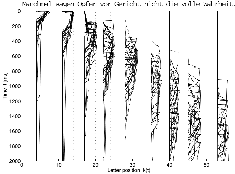
Figure 25: Temporal evolution of activations \{a_n(t)\} for N = 20 runs of the SWIFT model using sentence 17 of the Potsdam Sentence Corpus. The temporal evolution of the model induces a fast separation of activations between different runs.
