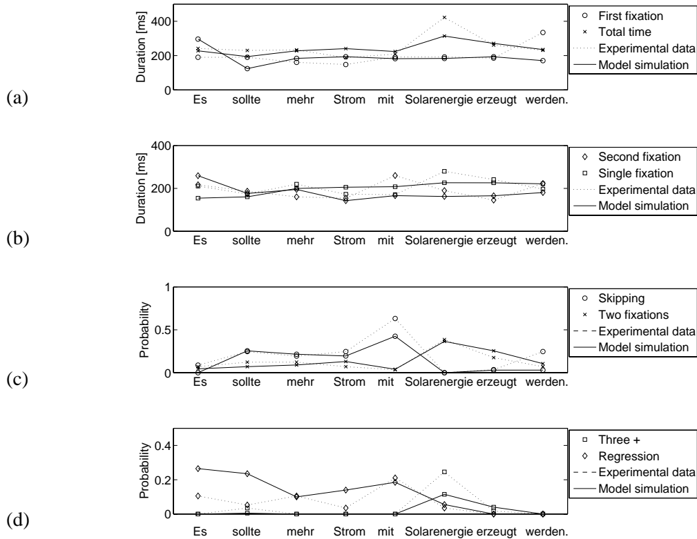
Figure 8: Example for the simulation results on the level of mean values over 200 runs of the model for 4 different measures of fixation durations (a,b) and 4 measures of fixation probabilities per word (c,d).
