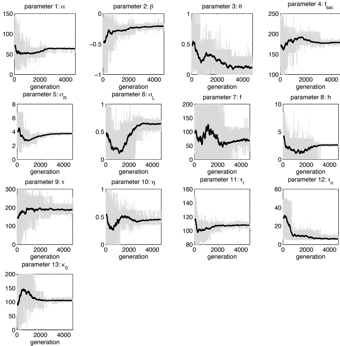
Figure 23: Evolution of parameter values in the optimization procedure by the genetic algorithm. The best value in each generation is indicated by the bold line, where errors are represented by the shaded areas. The shrinkage of errors indicated the convergence of parameter values in population of chromosomes.
