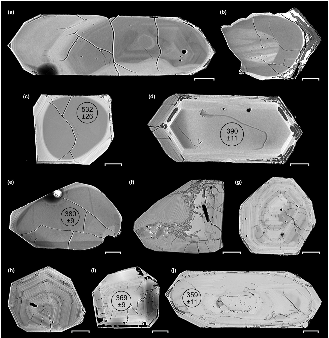
FIGURE 9 BSE images of zircons from sample Steina1: (a) A prismatic core with indistinct, concentric or sector zoning (Zrn1) is bounded on the left and lower sides by widely zoned, transgressive zircon, in turn overgrown by a finely zoned euhedral rim; grain no. 2. (b) An intermediate zone of homogeneous BSE-dark zircon (Zrn2) enclosing a planar-zoned multi-faceted core (Zrn1) has smoothly rounded interfaces with a finely zoned, altered rim; grain no. 16. (c) Finely zoned BSE-bright overgrowth (Zrn4) envelops a homogeneous, rounded, BSE-dark core (Zrn2); grain no. 4. (d) Prismatic crystal composed of homogeneous interior (Zrn3) and finely zoned concordant rims; grain no. 14. (e) Finely zoned overgrowth mantles an unzoned rounded core (Zrn3); grain no. 8. (f) A dissolution–reprecipitation reaction front propagating through homogeneous zircon produced the finely zoned zircon most common in sample Steina1; grain no. 17. (g) Patchy areas of homogeneous zircon persist in the core of a finely zoned euhedral crystal (Zrn4); grain no. 15. (h) A euhedral crystal (Zrn4) displays fine concentric zoning truncated by an overgrowth rim; grain no. 29. (i–j) Outer zones of euhedral crystals (Zrn4) and overgrowths are finely zoned, as opposed to absent or weak zoning in the core; grains no. 3 and 7. The circles show the location of laser spot analyses with concordant or near-concordant ^{206}\text{Pb}/^{238}\text{U} ages and 2\sigma error limits in million years. The dark and bright spots at grain margins in (a) and (e) are charging artefacts. Scale bar is 20 \mu\text{m}
