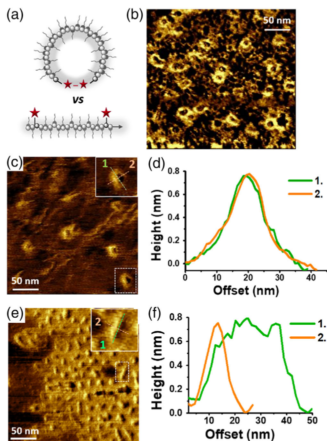
FIGURE 6 Schematic illustration of cyclic versus linear bottle brushes (A). AFM micrographs of crude c -P2 polymer with large fraction of free TAD-P n BuA 40 (B), purified c -P2 (C), and purified linear analogue l -P2 (E). Cross-section profiles of representative structures from C&E are provided in D&F (conditions: spin coating from CHCl 3 solution of 0.01 mg/mL brush concentration, freshly cleaved mica, phase image).
