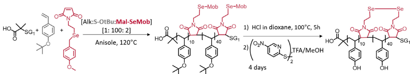
SCHEME 1 Synthetic route to polymers with positioned selenol entities for single chain folding by using NMP of 4- tert -butoxystyrene fed at suitable conversion with N -(2- para -methoxybenzyl selenoethyl) maleimide and subsequent folding by intramolecular diselenide bridge formation.
