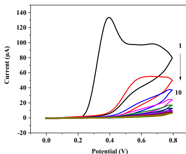
Figure 2. Cyclic voltammograms recorded between 0 and 0.8 V/s during the electropolymerization of o -PD on the GCE for MIP synthesis ( 5 mM o -PD and 25 \mu\text{g/mL} BuChE, in 100 mM acetate buffer pH 5.2 , 50 mV/s, 10 cycles).
