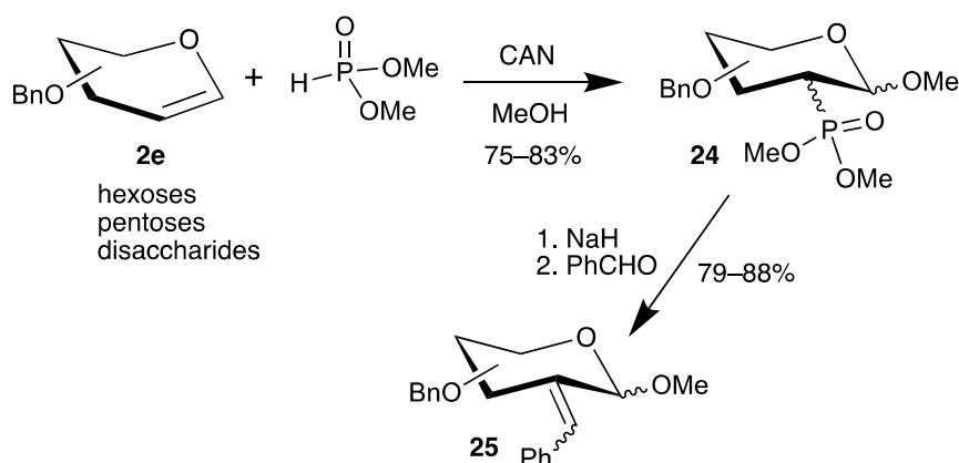
Scheme 12. Addition of dimethyl phosphite to benzyl-protected glycals 2e in the presence of CAN and subsequent Horner–Emmons reaction.
