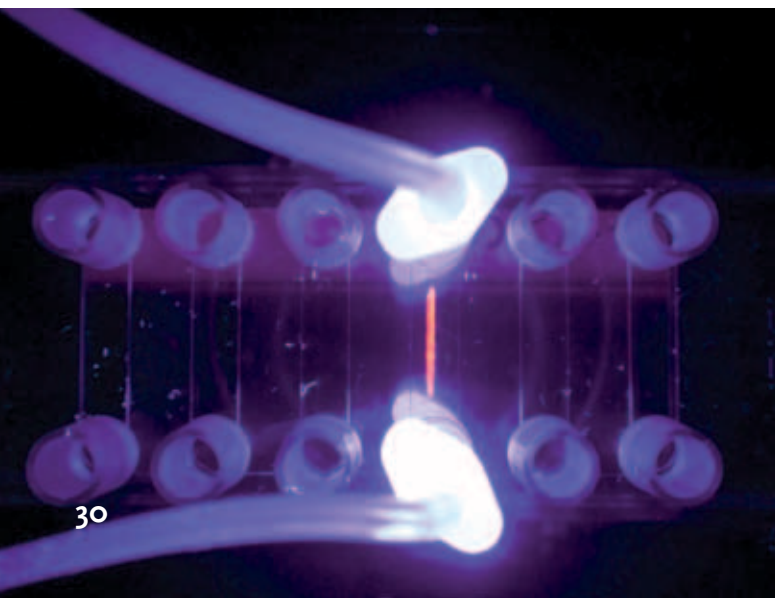
Microchannels prepared with oxygen sensors of Colibri Photonics
