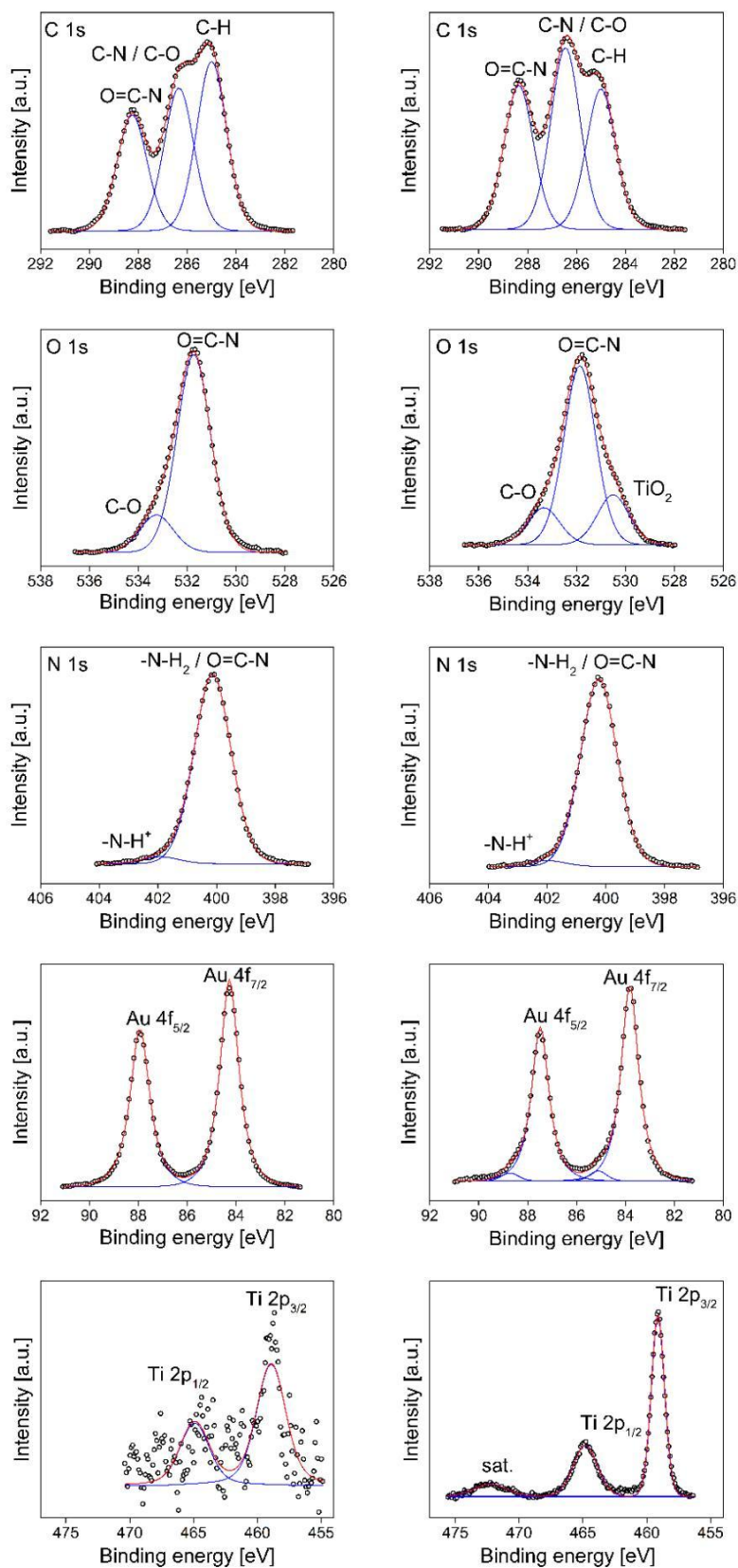
Figure 5: Au 4f, Ti 2p, C 1s, N 1s, and O 1s XP spectra of the TS Au2.5 (left) and TPS Au2.5 (right) surfaces. Open circles are experimental data, red line represents the sum of all fits and blue lines are the single fit components.
