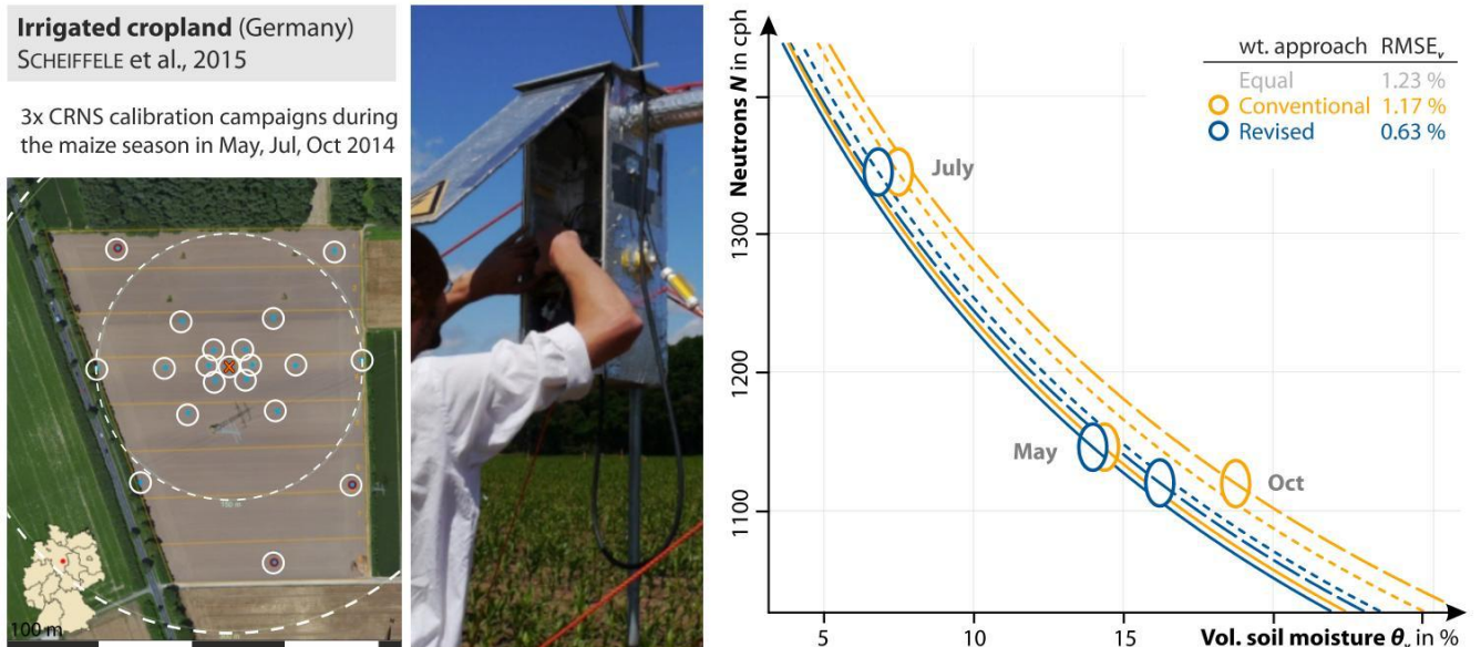
Figure 6. Recalibration of the CRNS sensor in an agricultural maize field (Braunschweig, Germany). Sizes of the circles indicate the corresponding uncertainty range of the measurement, while every such measurement corresponds to a calibration curve \theta(N, N_0) . The conventional weighting approach is not able to provide a unique theoretical line through the 3 calibration days. Furthermore, for a given neutron observation the difference between estimated moisture (lines) and actual soil moisture (ellipses) indicates unrealistic biomass dynamics throughout the study period (see explanations in the text). The revised approach converges the datasets to confirm the accepted neutron theory almost in a single calibration curve within uncertainties (size of ellipses).
