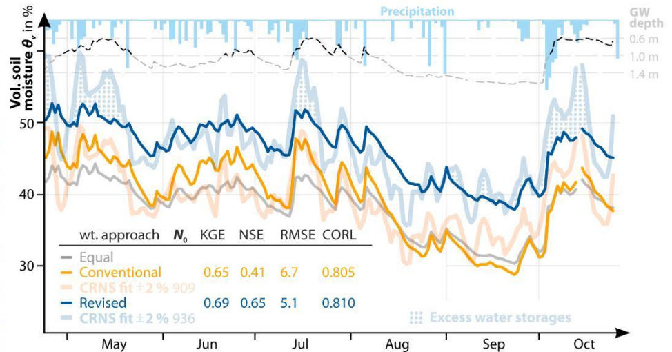
Figure 9. Time series of CRNS soil moisture and groundwater at the Wüstebach forested river catchment. Fitting the CRNS data to the SoilNet conventional average almost completely hides effects from excess water storages (which could include water in the litter layer, interception water, groundwater rise, or ponding close to the stream). The revised approach emphasizes those additional hydrological processes while still robustly increasing the sensor performance.
