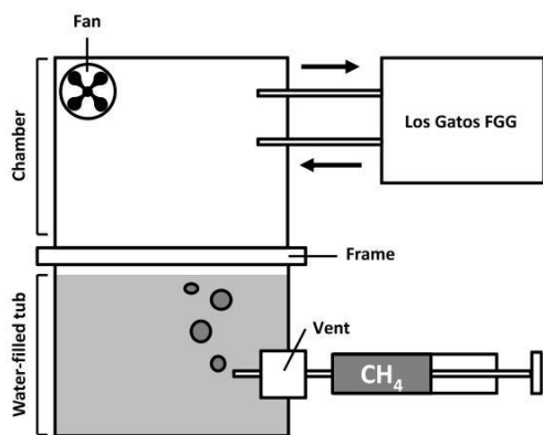
Figure 4. Scheme of experimental setup used for the simulation and determination of ebullition events with a Los Gatos fast greenhouse gas (FGG) analyser (911-0010, Los Gatos). The crimped area represents water-filled tub.
