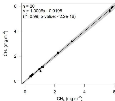
Figure 5. Scatter plot of the amount of injected CH 4 and the corresponding calculated CH 4 ebullition event. The solid black line indicates the 1 : 1 agreement. The linear fit between the displayed values is represented by the black dashed line, surrounded by the 95 % confidence interval (grey shaded area).
