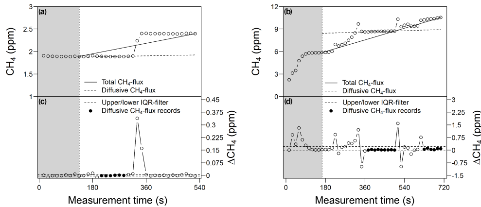
Figure 3. Time series plot of recorded concentrations (ppm) within the chamber headspace for (a) a simulated ebullition event and (b) an exemplary field study CH 4 measurement. Time spans dominated by diffusive CH 4 release are marked by (c, d) black dots, enclosed by the 25 and 75 % quantiles \pm 0.25 IQR of obtained concentration changes, shown as black dashed lines. Unfilled dots outside the dashed lines display ebullition events (see also Goodrich et al., 2011; Miller and Oremland, 1988). Grey shaded areas indicate the applied death band at the beginning of each measurement (25 %). Negative \Delta\text{CH}_4 values indicate a overcompensation due to (temporally) insufficient headspace mixing.
