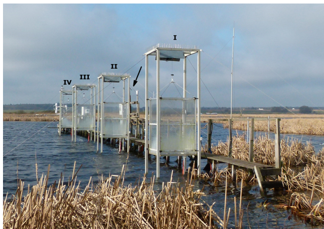
Figure 1. Transect of automatic chambers (ACs) established at the measurement site. The arrow indicates the position of the climate station near chamber II.
