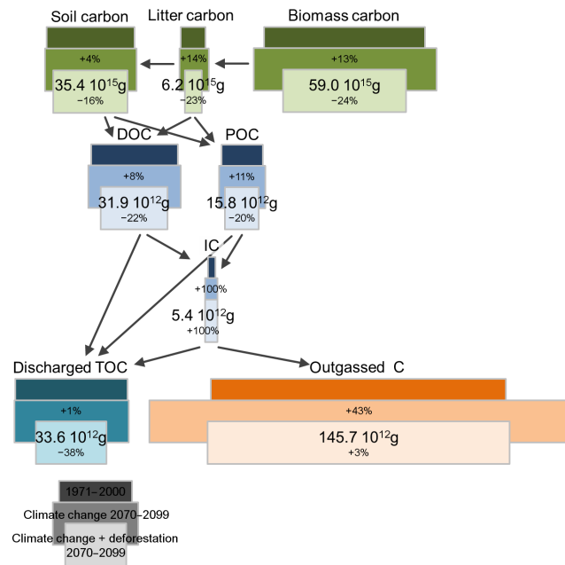
Figure 4. Averaged annual amounts and change in the basin carbon budget due to climate change and deforestation. Dark boxes indicate the amount of carbon during the reference period (1971–2000), intermediate boxes during the future period (2070–2099) under climate change only (Langerwisch et al., 2016), light boxes during the future period under the forcing of climate change and deforestation (BAU) together (average over all SRES scenarios and GCMs). Amount is given for future period with relative change compared to reference. Arrows indicate the direction of carbon transfer.
