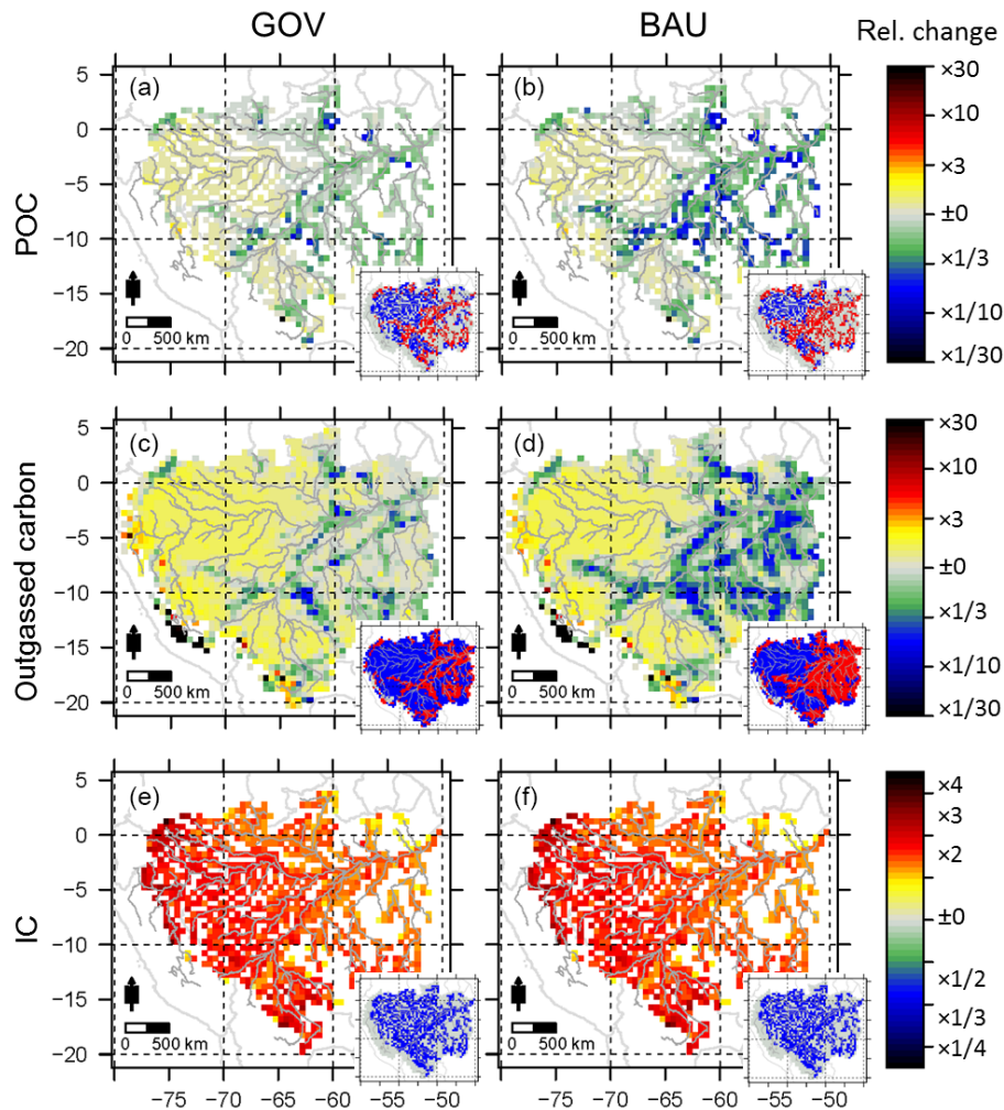
Figure 5. Change in carbon caused by deforestation and climate change. Climate model mean ( E_{CCDefor} ) of the change of particulate organic carbon POC (a, b), outgassed carbon (c, d) and inorganic carbon IC (e, f). The inset maps show blue areas where changes are predominantly caused by climate change ( D_{CC} ) and red areas where changes are predominantly caused by deforestation ( D_{Defor} ). For further details see Fig. 3. White areas within the Amazon basin represent cells where changes are not significant ( p value > 0.05).
