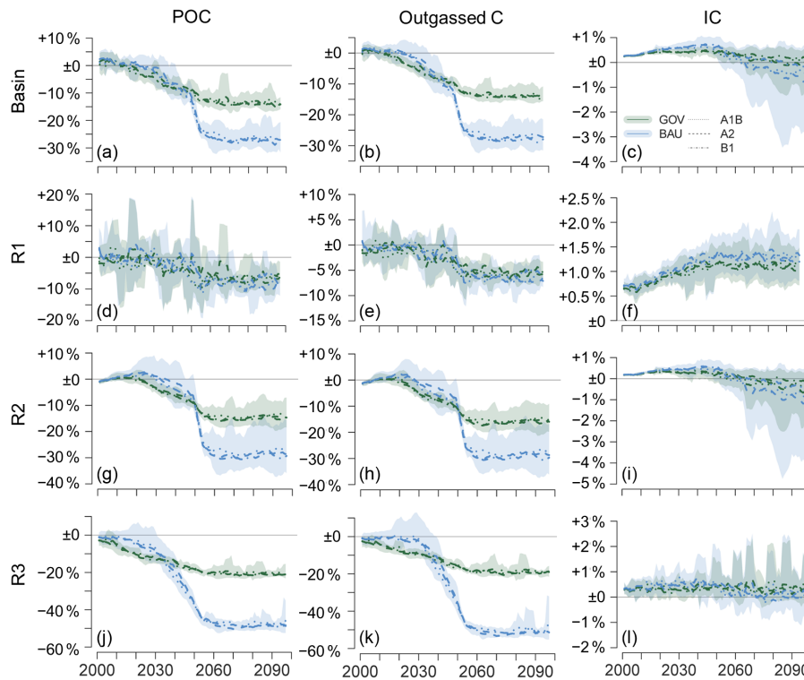
Figure 6. Temporal change in riverine organic carbon due to land use change only. Change of annual sum of carbon in the deforestation scenario (GOV or BAU) compared to the NatVeg scenario for the whole basin (a–c) and the three subregions (R1–R3; d–l) as 5-year mean for GOV (green) and BAU (blue), representing E_{\text{Defor}} . The shaded areas indicate the full range of values of all five climate models. Bold lines represent the 5-year mean of the five climate models.
