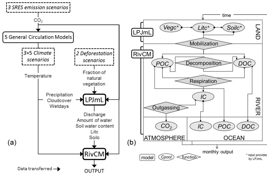
Figure 1. Overview of the general transfer of data between scenarios and models (a) and the detailed calculation of carbon fluxes within and between LPJmL and RivCM. (b).
