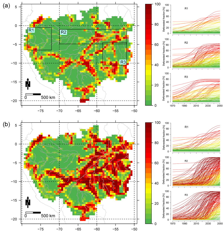
Figure 2. Fraction of deforested area per cell (%) in 2050. Data are based on Soares-Filho et al. (2006). (a) refers to the BAU deforestation scenario, whereas (b) refers to the GOV scenario. The three subregions discussed in the main text are highlighted in the map. The timelines (right panels) show the development until 2050 for each subregion (deforestation kept constant after 2050).
