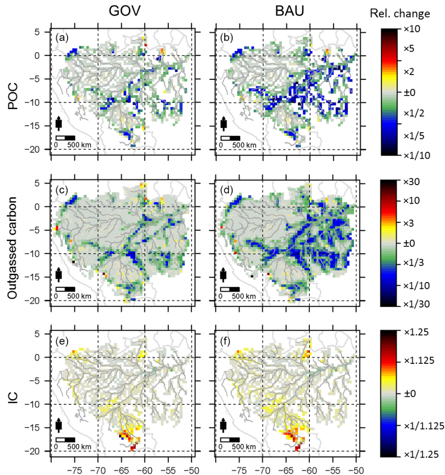
Figure 3. Change in carbon caused by deforestation. Climate model mean ( E_{\text{Defor}} ) of the change of particulate organic carbon POC (a, b), outgassed carbon (c, d) and inorganic carbon IC (e, f). Results of the SRES emission scenario A1B are averaged over five climate models. Areas in yellow and red indicate a gain, and areas in green and blue indicate a loss in carbon caused by deforestation (GOV and BAU). White areas within the Amazon basin represent cells where changes are not significant ( p value > 0.05).
