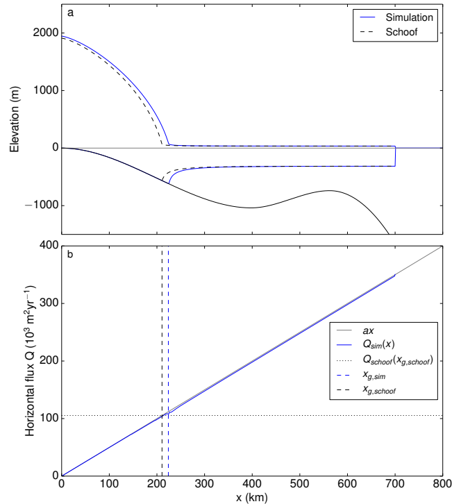
Figure A2. (a) Comparison between the semi-analytical ice-sheet profile from Schoof and our modeling result for the final steady-state ice sheet of simulation BC0 (only the RHS of the symmetric ice sheet is shown here). Panel (b) shows Schoof's and the modeled grounding line position, x_{g,schoof} = 211 km and x_{g,sim} = 224 km, respectively, as well as the steady-state ice flux from simulation, Q_{sim}(x) , along the model domain to compare with ax and the analytically derived Schoof flux, Q_g , at x_{g,schoof} .
