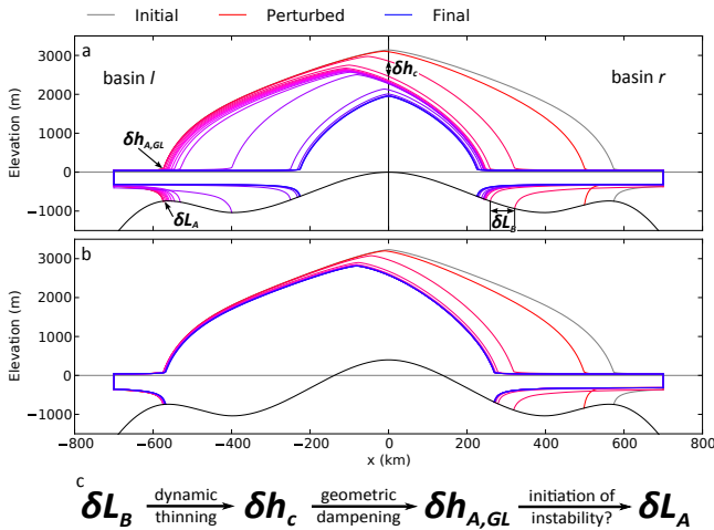
Figure 4. Profiles of the transient ice sheet between the end of perturbation (red), and the final steady state (blue) for two different values of central bed elevation (a) b_c = 0 m (example of unstable scenario U, same as in Fig. 3a) and (b) b_c = +400 m (example of stable scenario S). The time interval between two consecutive profiles is 1 kyr. (c) explains the mechanism of basin interaction conceptually with the notation depicted in panel (a).
