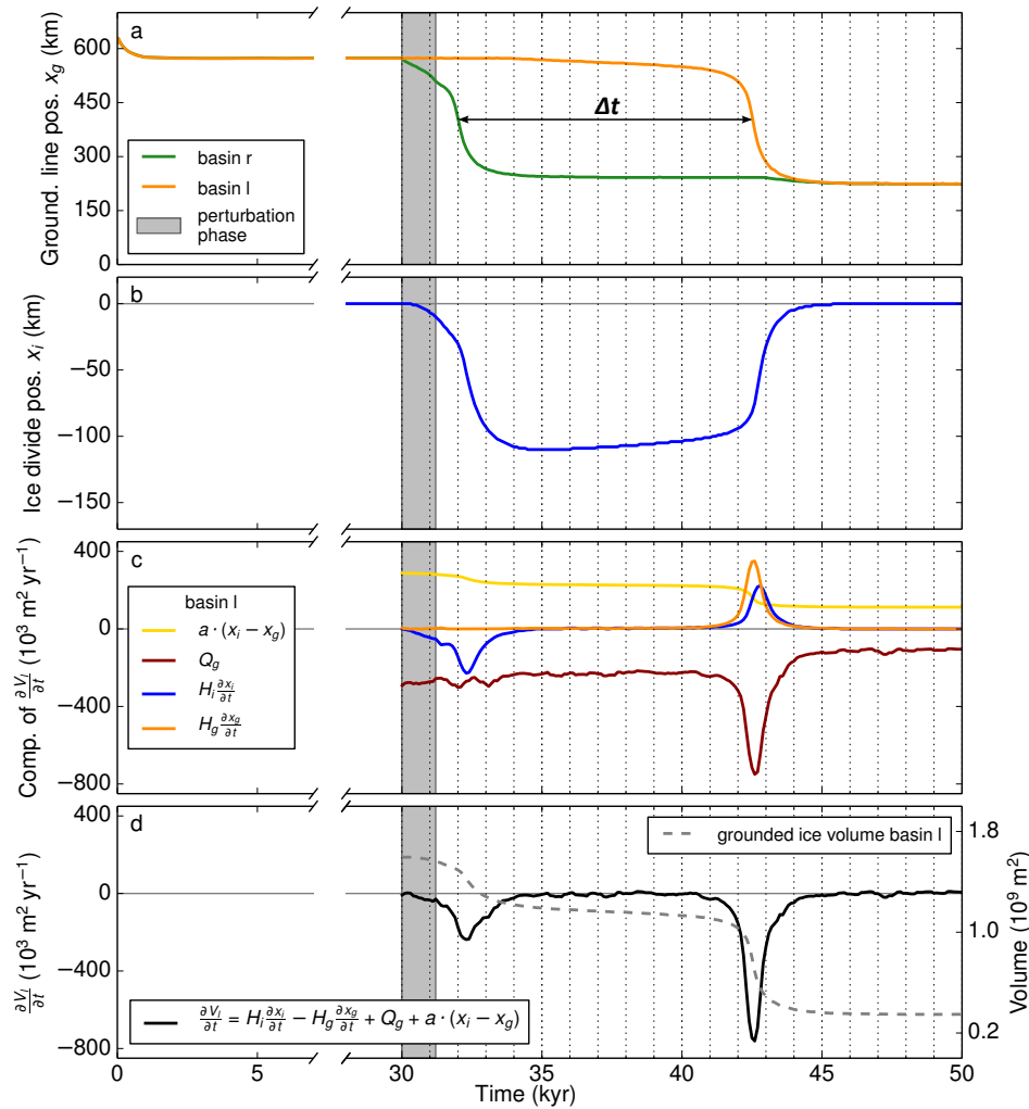
Figure 5. Time series for the unstable scenario U (simulation BC0, see Figs. 3a and 4a) of (a) the absolute value of the grounding line positions (b) the position of the ice divide (as defined in the text), (c) the individual components of \frac{\partial V_I}{\partial t} (as derived in Sect. 3.1, smoothed with a 500-year moving window), (d) the sum of these components and the grounded ice volume of basin I. The transition time \Delta t , used in Eqs. (8)–(10), is depicted by a double-headed arrow in (a).
