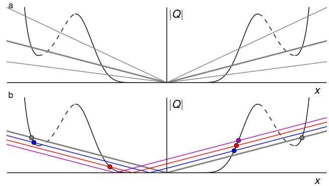
Figure 8. Conceptual picture to identify steady-state grounding line positions and analyze basin stability. The grounding-line flux Q_g (black curve) according to Eq. (1) is shown for a symmetric, overdeepened bed shape used in our experiments. The dashed lines mark the sections of retrograde bed. (a) Different gray lines show the mass gain through snowfall, ax , for a symmetric ice sheet for three different magnitudes of surface accumulation a . Intersections of Q_g and ax yield possible steady-state grounding line positions. (b) Colored lines give a(x - x_i) for one accumulation magnitude (thick line in panel a) but different positions of the ice divide, x_i , that is shifted leftward in response to an assumed destabilization of basin I. Grounding line positions (circles) are shown for the three scenarios S (blue), U (red) and C (purple) discussed in this study as well as an initial symmetric steady state (gray).
