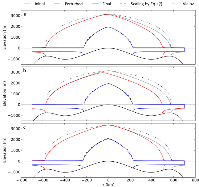
Figure A1. Ice-sheet profiles at three stages of simulation for a central bed elevation of b_c = 0 m with applied (a) oceanic (same as Fig. 3a) and (b) atmospheric perturbation. Panel (c) shows a set of SSA only simulations using an oceanic perturbation.
