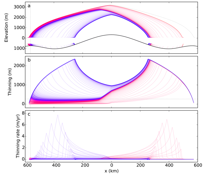
Figure 10. Ice-sheet (a) profile, (b) thinning with respect to the ice thickness at the end of perturbation and (c) thinning rate at multiple stages (time interval 100 years) of the unstable scenario U (simulation BC+330). The ice shelf is truncated for better visibility. The vertical dotted line indicates the location of maximum sill elevation x_{-s} . The horizontal dotted line in panel (b) gives the amount of cumulative thinning necessary to cause the ice situated on the local bed maximum to become afloat. The same color-coding as in Fig. 4 applies.
