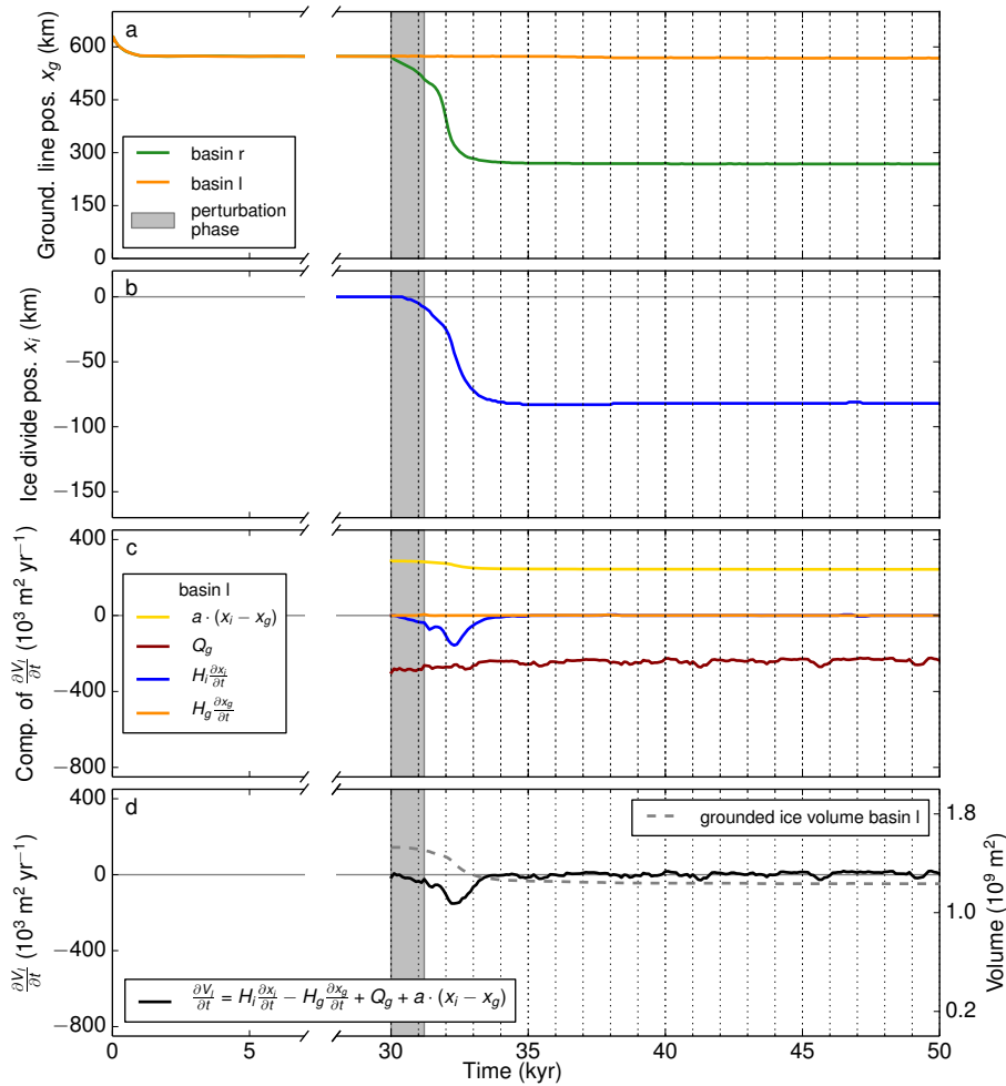
Figure 6. Same as Fig. 5 but here for the stable scenario S (simulation BC+400, see Fig. 4b).
