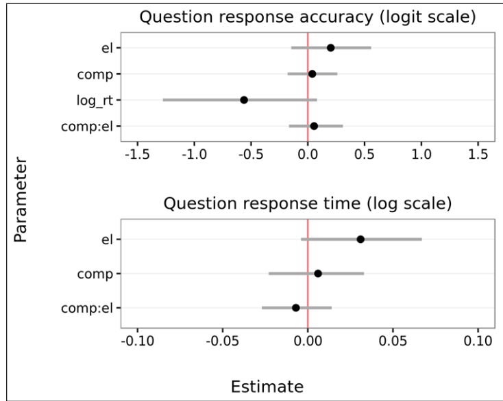
Figure 2: Experiment 1 – Question response times and accuracies: caterpillar plot of means and 95% credible intervals for parameters of interest. el = elision, comp = complexity, log_rt = log response time.
