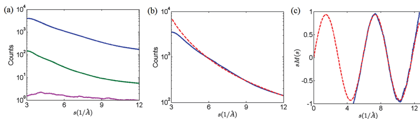
Fig. 4 Diffraction intensity of static \text{N}_2 molecules. (a) Azimuthally averaged diffraction intensity (blue), background taken without gas (green) and background taken without electron beam (magenta). The vertical axis is the raw camera counts per pixel per one minute integration time. (b) Azimuthally averaged diffraction intensity of static \text{N}_2 molecules (blue solid) and the scattering background obtained by a standard fitting routine (red dashed). (c) Experimental (blue solid) and simulated (red dashed) modified diffraction intensity sM(s) . (c) is adapted from ref. 1
