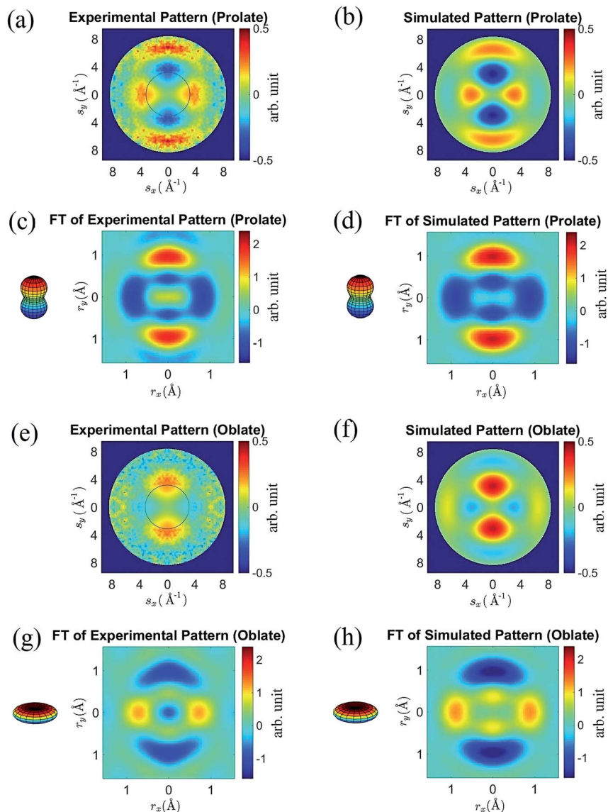
Fig. 7 2D \text{N}_2 diffraction patterns at half revival. (a) Experimentally measured and (b) simulated diffraction-difference patterns of the prolate distribution. (c) and (d) are Fourier transforms of (a) and (b), respectively. (e) Experimentally measured and (f) simulated diffraction-difference pattern of the oblate distribution. (g) and (h) are Fourier transforms of (e) and (f), respectively. In patterns (a) and (e), the data inside the black circles are missing due to the beam stop. They are obtained by extrapolating the pattern and letting the counts smoothly go to zero towards the center. For illustrative purpose, angular distributions are shown on the side of panel (c), (d), (g) and (h) for visual guidance. Figure is reproduced from ref. 1.
