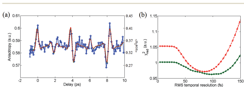
Fig. 6 Experimental anisotropy and \chi^2 fitting. (a) Anisotropy evolution from experimental data (blue circles), simulation with values from the 2-parameter fit (dashed red line), and simulations with values from the 4-parameter fit (solid green line). (b) The reduced \chi^2 metric for the 4-parameter fit (circles and solid green line) and 2-parameter fit (circles and dashed red line). The 4-parameter fit involves laser fluence, initial temperature, temporal resolution and a re-scaling factor that accounts for the excitation percentage of the target molecules. The 2-parameter fit uses the measured laser fluence and estimated initial temperature, while varying the temporal resolution and the re-scaling factor. The optimal temporal resolution from the 4-parameter fit and 2-parameter fit are 100 fs RMS and 85 fs RMS, respectively.
