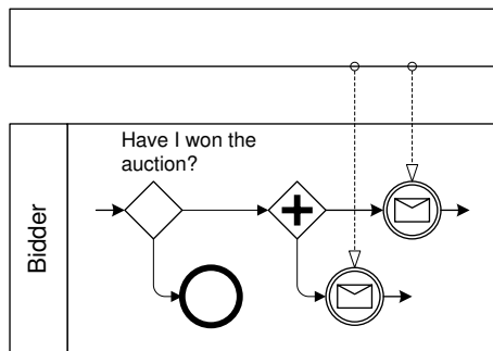
Figure 4.25: D2. Impossible data-based decisions
