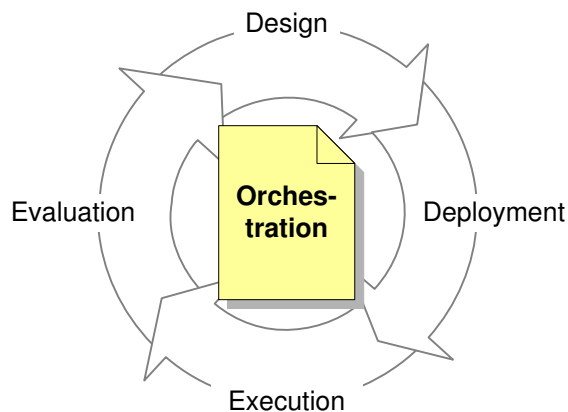
Figure 2.2: Orchestration Lifecycle
