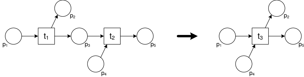
Figure 5.7: Transition aggregation
