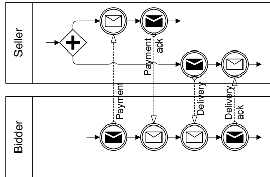
Figure 4.29: O3. Uni-lateral sequentialization
