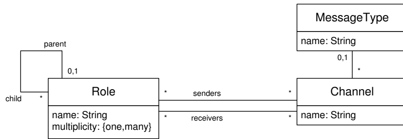
Figure 5.20: Meta-model for role-based models
