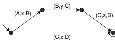
Figure 5.41: Unfolding of the acyclic interaction model
