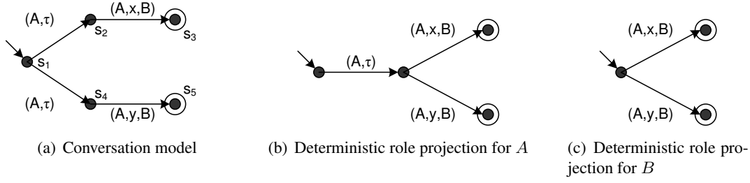
Figure 5.3: Deterministic role projections
