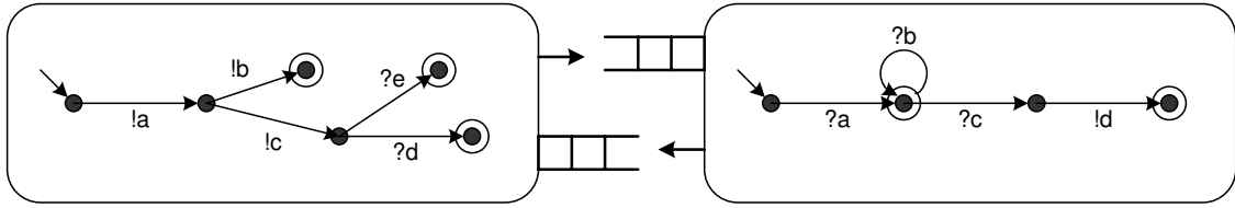
Figure 2.9: Communicating Finite State Machine example
