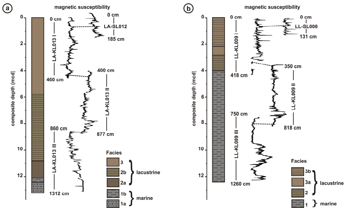
Figure 4.3: Lithological units and splice construction based on magnetic susceptibility. (a): Lago Lanahue master core (composed of gravity-core LA-SL012 on top and piston-core LA-KL013 below). (b): Lago Lleu Lleu master core (composed of gravity-core LL-SL008 on top and piston-core LL-KL009 below). Please note: the depth in cm given for single core sections is the depth that was used during drilling operations; the composite depth in mcd (meter composite depth) is the depth resulting from splice construction.
