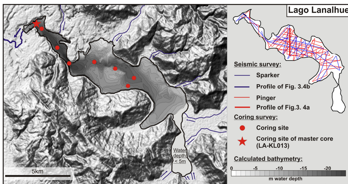
Figure 3.4a: Bathymetry, coring positions, and seismic survey lines of Lago Lanalhue. Bathymetry calculated using seismic profiles; isobath every 1 m.
