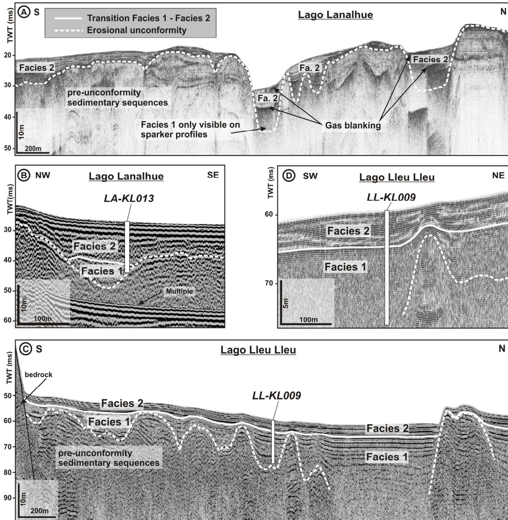
Figure 3.5: Seismic profiles of Lago Lanalhue and Lago Lleu Lleu. The position of the respective seismic lines is indicated in Figure 3.4 (a+b). The unconformity, stratigraphic boundary, and core-to-seismic correlation are shown. A: S-N pinger profile in the central part of Lago Lanalhue. B: NW-SE sparker profile with projection of LA-KL013. C: S-N sparker profile in the central part of Lago Lleu Lleu with projection of LL-KL009. D: Pinger profile with projection of LL-KL009.
