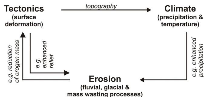
Figure 1.1 Schematic diagram of processes and their feedbacks working at convergent plate margins (modified after Willet et al., 2006)
