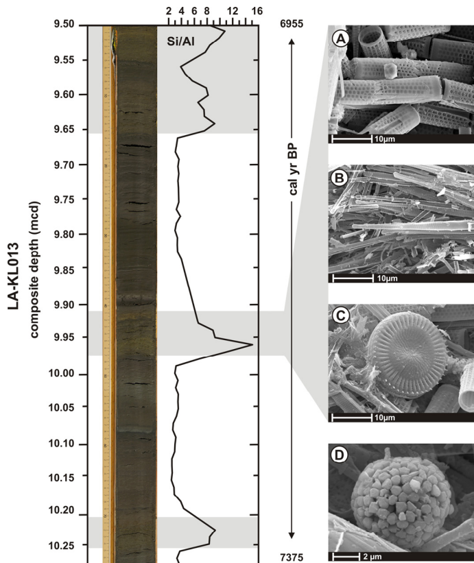
Figure 4.6: Left: Comparison of the Si/Al ratio of the sediments and the occurrence of diatom-rich layers (highlighted in grey) in sediment core LA-KL013. Right: SEM-images of the most abundant diatoms and present framboidal pyrite.
