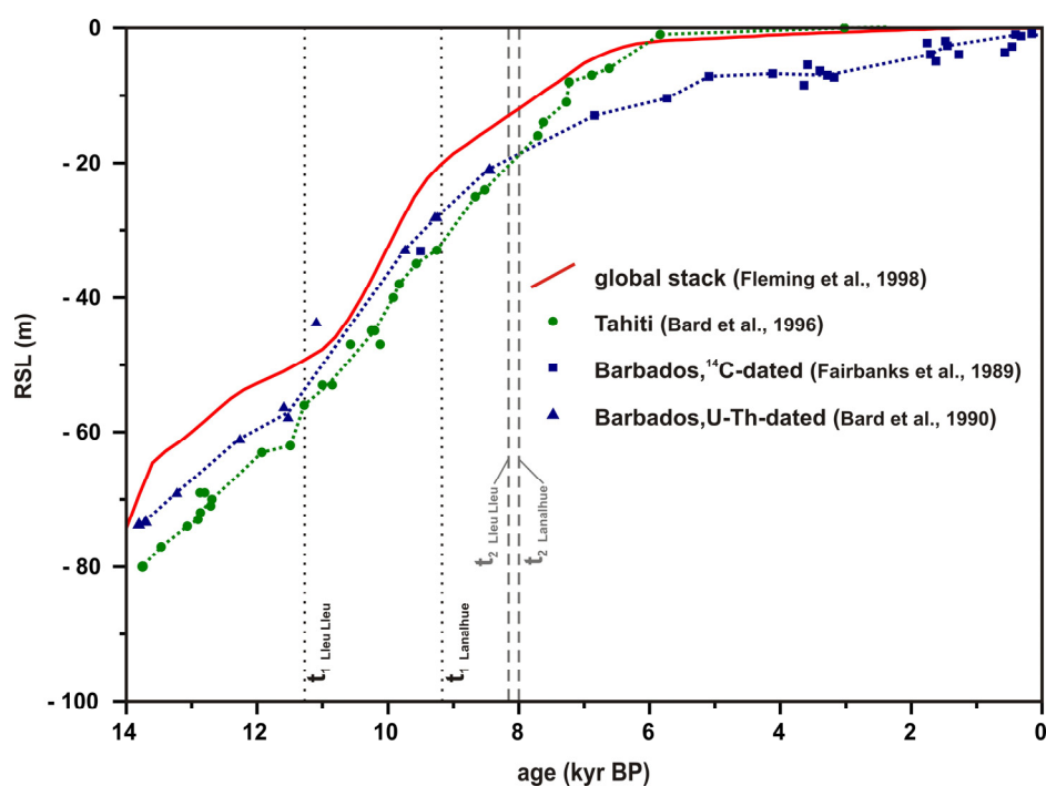
Figure 3.8: Comparison of the different Holocene sea-level curves used for the calculation of uplift rates: the global stack of Fleming et al. (1998) (red line), the Tahiti coral record of Bard et al. (1996) (green dotted line + dots), the ^{14}\text{C} -dated Barbados coral record of Fairbanks et al. (1989) (blue dotted line + squares), and the U-Th-dated Barbados coral record of Bard et al. (1990) (blue dotted line + triangles). The timing of Transition 1 ( t_1 , black dotted line) and Transition 2 ( t_2 , grey dashed line) is indicated for Lago Lanalhue and Lago Lleu Lleu, respectively.
