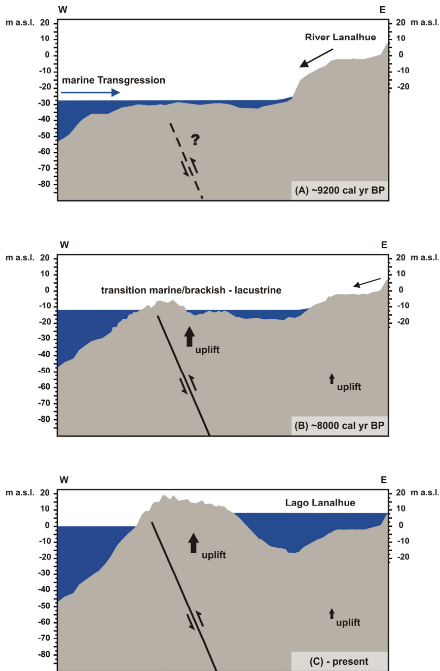
Figure 3.7: Model of the lake development, exemplary shown for Lago Lanalhue (not to scale). Elevation (m a.s.l.) relative to present sea level. (A) At 9200 cal yr BP, the valley of the former River Lanalhue was drowned by the marine transgression for the first time; depositional conditions were marginal marine to brackish. (B) At 8000 cal yr BP, the swell was uplifted above the global sea level; the marginal marine/brackish conditions changed into lacustrine ones. (C) At present, Lago Lanalhue is impounded behind the uplifted swell.
