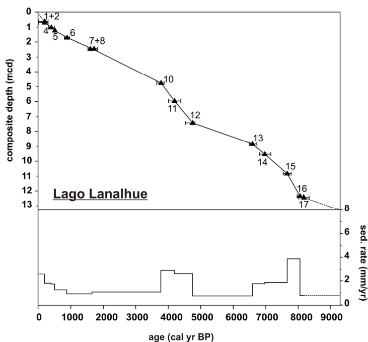
Figure 4.4a: Age-depth relationship and calculated sedimentation rates of the Lanalhue master core (LA-KL013). Numbering of single dating points refers to Table 4.2a. Grey dots are indicating non-fitting ages which were neglected for the age model. For the calculation of sedimentation rates, the mean of ages 1+2 and 7+8 was taken to avoid unnatural high sedimentation rates caused by the close sample spacing.
