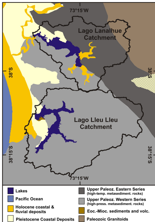
Figure 4.2: Simplified geologic map of the Lanalhue and Lleu Lleu catchment regions (catchments framed by the solid black line); modified after Melnick et al. (2009).
