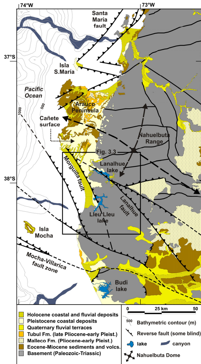
Figure 3.2: Simplified geologic map of the Arauco-Nahuelbuta region (modified after Melnick et al., 2009). The Arauco Peninsula as an uplifted part of the continental shelf is well distinguishable from the Paleozoic-Triassic basement of the Nahuelbuta Range.
