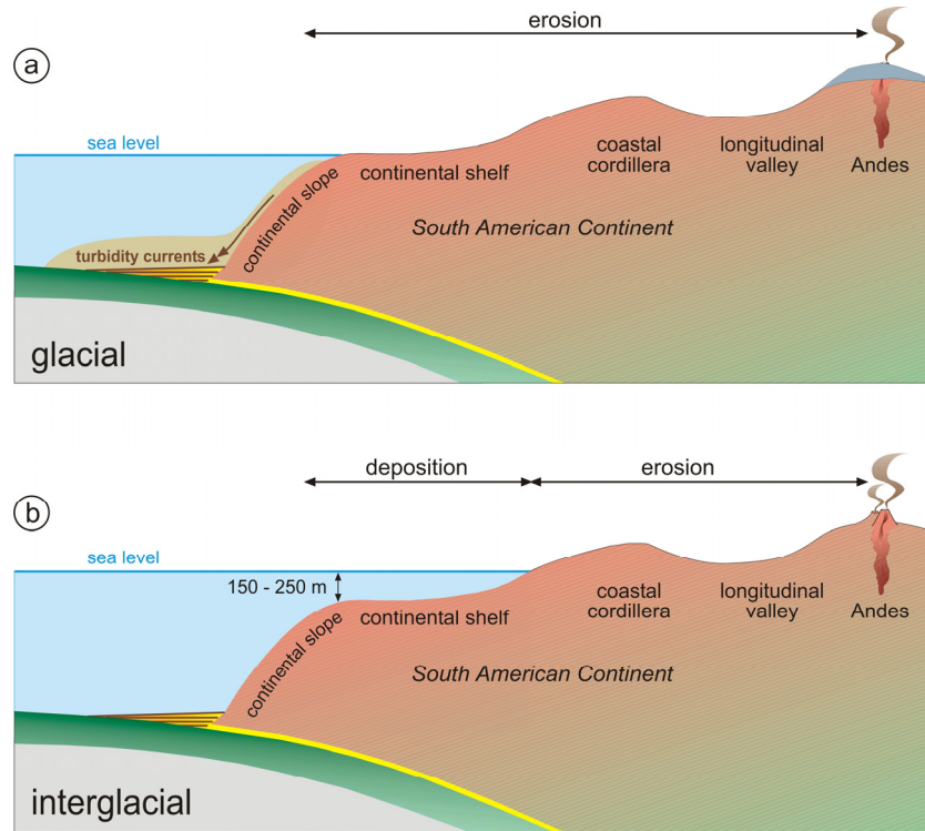
Figure 2.7: Schematic representation of a glacial and an interglacial scenario (not to scale). (a) Glacial period with lowered sea level and exposed continental shelf. The shelf is being eroded and the accumulation space for sediments is reduced; that way, sediment is bypassing the shelf area. Turbidity currents occur frequently. (b) Interglacial period with a high sea level and drowned continental shelf. The shelf region acts as depositional center for terrestrial sediments. Turbidity currents are occurring sporadically.
