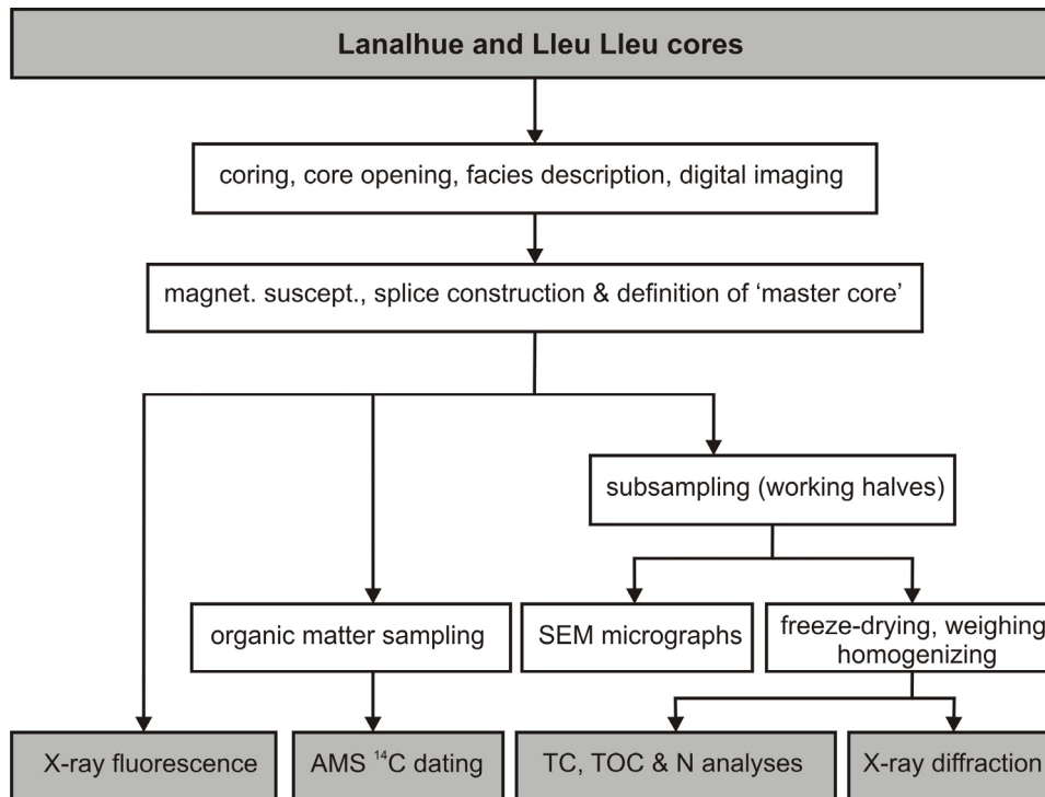
Figure 1.7 Operation chart for the lacustrine sediment records of Lago Lanalhue and Lago Lleu Lleu
