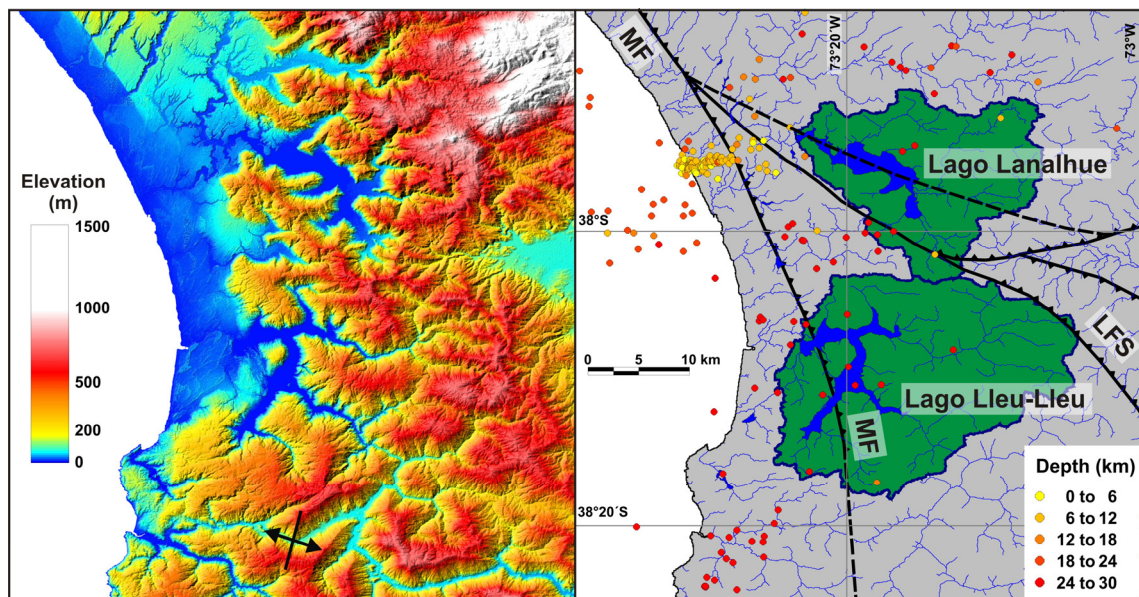
Figure 3.3: Topography, seismicity and local river network in the direct vicinity of Lago Lanalhue and Lago Lleu Lleu. Left: Shaded topography (SRTM, NASA). The black arrow marks the tectonically induced flow reversion of the Pellahuén River (according to Rehak et al., submitted). Right: Depth-colored seismicity according to the ISSA (Bohm et al., 2002; Bruhn, 2003; Bohm, 2004) and TIPTEQ (Haberland, 2006) networks. Green-shaded areas mark the drainage basins of the lakes. MF = Morguilla Fault (blind thrust, not outcropping; northern part after Melnick et al., 2009), LFS = Lanalhue Fault System (Glodny et al., 2008).
