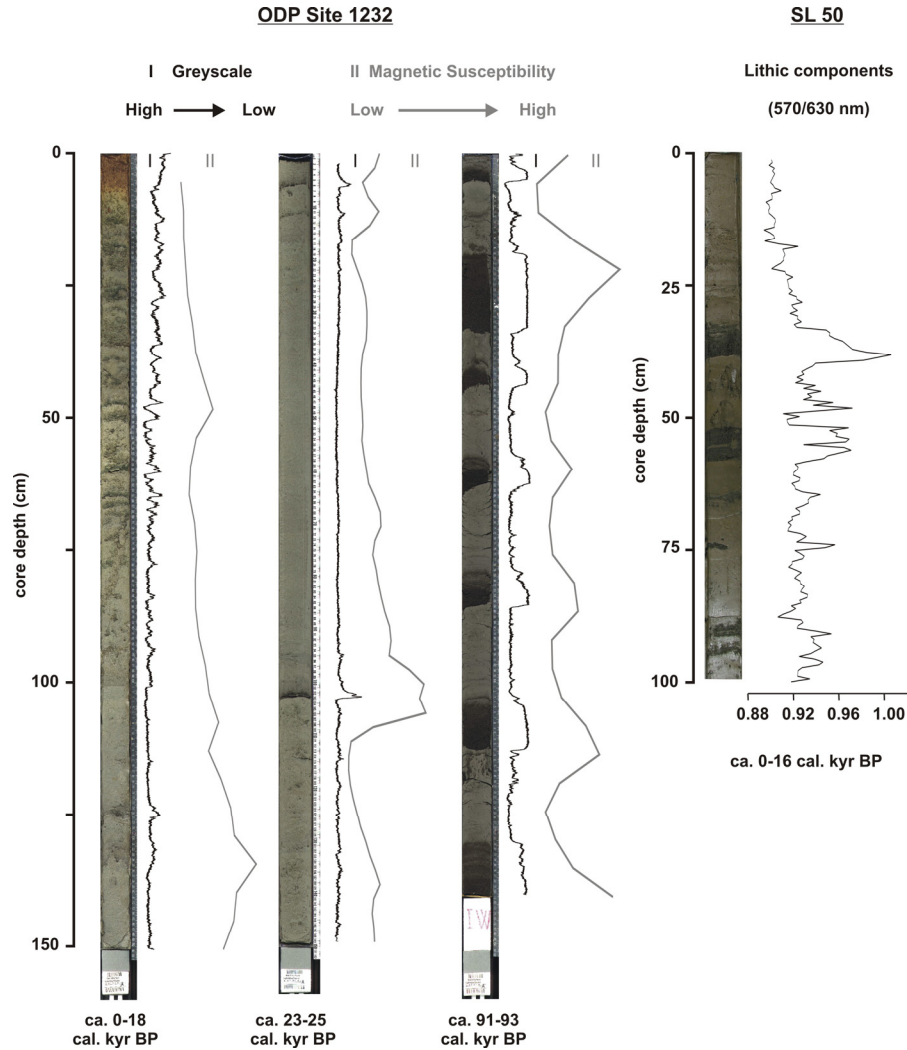
Figure 2.3: High-resolution greyscale data profile of ODP core 1232 derived from core photography and magnetic susceptibility data measured onboard with a Multisensor Core-Logger at 5-cm intervals (Mix et al., 2003). Both parameters display distinctly different values for the turbiditic layers and for the hemipelagic layers and are, thus, used for the quantification of the turbidites. Turbidites of core SL 50 were identified by means of colour scanning with a Spectrolino scanner; the ratio of the reflectance at 570 nm over that of 630 nm provides a proxy for lithic sediment components (Rein and Sirocko, 2001; Rein, 2003).
