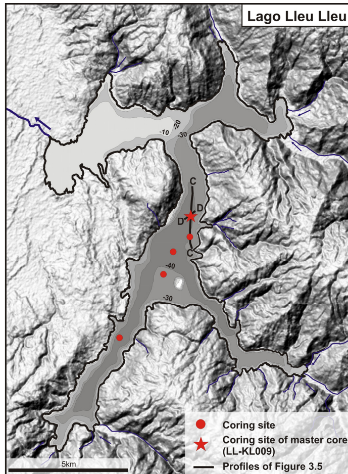
Figure 3.4b: Bathymetry and coring positions of Lago Lleu Lleu. Bathymetry derived from Urrutia et al. (2000); isobath every 10 m.
