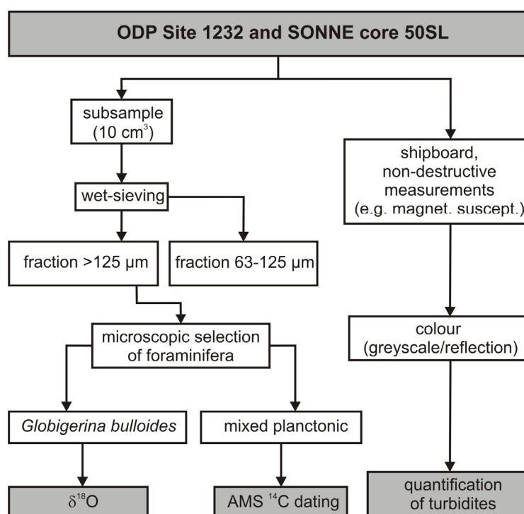
Figure 1.6 Operation chart for the marine sediment records ODP Site 1232 and SONNE core 50SL
