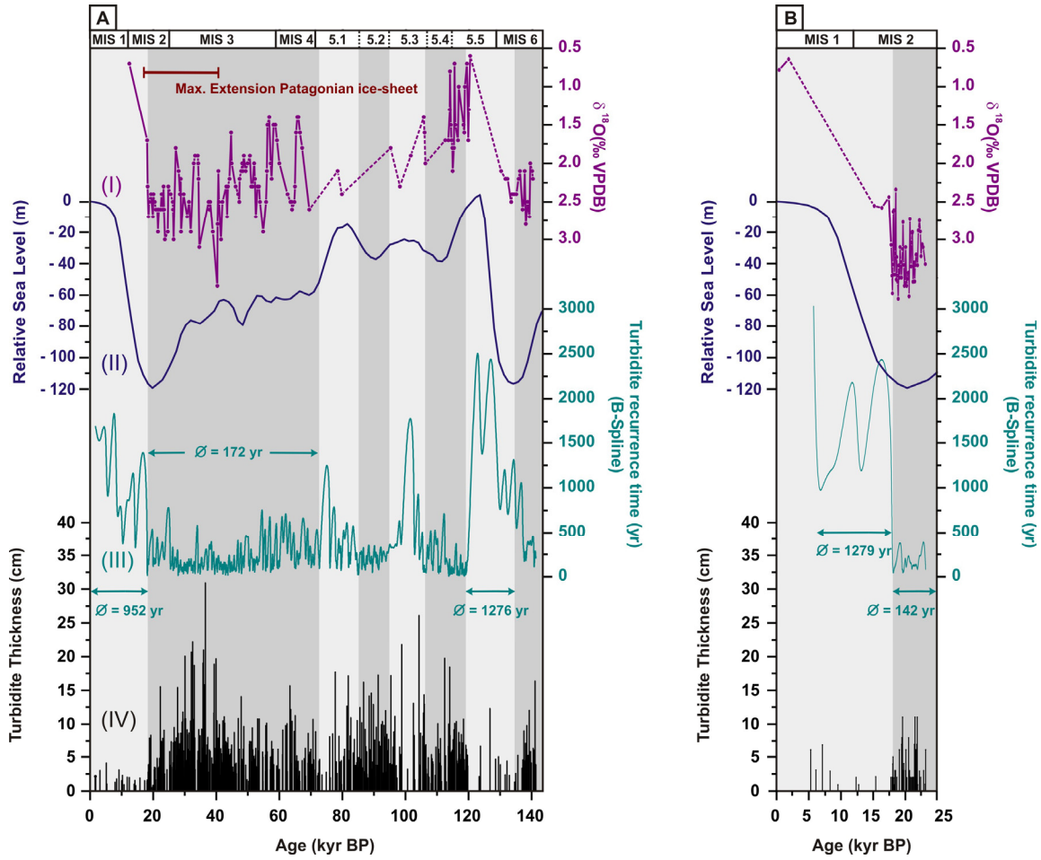
Figure 2.5: Turbidite and oxygen isotope records of ODP Site 1232 (A) and SONNE core 50SL (B) compared to the global sea level record for the past 140 kyr. (I) Oxygen isotope record ( \text{‰VPDB} ), (II) global sea level record (after Waelbroeck et al., 2002), (III) calculated turbidite recurrence time (kyr) displayed as B-Spline, (IV) thickness of turbiditic layers (cm). Light gray bars highlight episodes of long turbidite recurrence times during periods of sea level highstand and during terminations; darker gray bars highlight episodes of short turbidite recurrence times during periods of low sea level. The period of maximal Patagonian ice sheet extension is indicated by the brown bar at the top of the graph.
