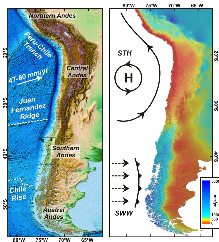
Figure 1.3 Climatic and tectonic setting at the Andean margin of South America. Left: Bathymetry and topography along the Chilean convergent margin (map source: ETOPO1 Global Relief Model; Amante and Eakins, 2008); major tectonic structures of the oceanic plate and the trench system are highlighted in white; plate convergence rate after Angermann et al., 1999 and Kendrick et al., 2003. Right: Mean annual precipitation (data from New et al., 2002); the present-day positions of the Subtropical High Pressure Cell (STH) and the Southern Westerly Winds (SWW) are indicated.
