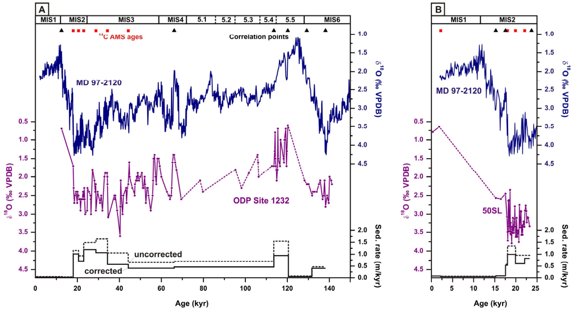
Figure 2.4: Correlation of the ODP Site 1232 (A) and SONNE core 50SL (B) oxygen isotope records with the oxygen isotope record of core MD 97-2120 (Pahnke et al., 2003). All data sets are based on planktonic foraminifera ( Globigerina bulloides ). Red quadrates are indicating AMS ^{14}\text{C} dating points; black triangles are indicating oxygen isotope correlation points. Dashed parts of the ODP and SONNE graphs correspond to sections with insufficient amounts of foraminifera. The sedimentation rate was calculated for the whole sedimentary sections including turbiditic layers (uncorrected – dashed line) as well for the hemipelagic sections excluding the turbidites (corrected – solid line).
