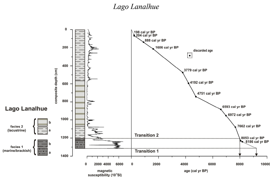
Figure 3.6a: Lithological units, magnetic susceptibility values and age model of the Lanalhue master core LA-KL013. Facies 1 (dark-grey) is of marine/brackish, facies 2 (light-grey) of lacustrine origin. The facies transitions are indicated with dashed lines/arrows. All dating results, except one age, are in stratigraphic order; the non-fitting age is marked by the dashed square and ignored for the age model.
