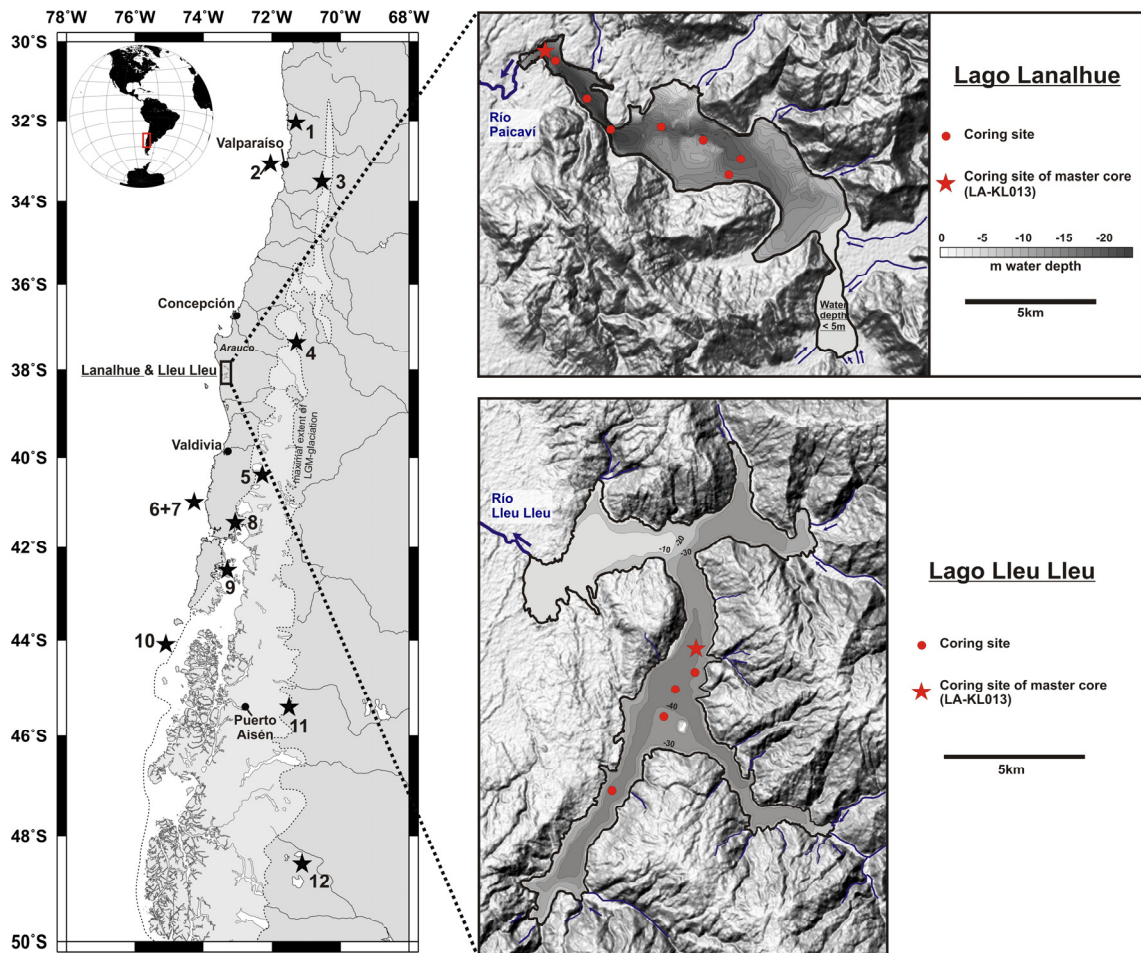
Figure 4.1: Position of Lago Lanalhue and Lleu Lleu at the south-central Chilean margin. Left: Extended study area and locations of adjacent studies discussing Holocene paleoclimatic and –environmental changes (black stars). 1: Palo Colorado Swamp Forest (Maldonado and Villagrán, 2006), 2: marine sediment core GeoB 3302-1 (Lamy et al., 1999) 3: Laguna Aculeo (Jenny et al., 2002a and b, Villa-Martínez et al., 2003), 4: Lago Laja (Torres et al., 2008), 5: Lago Puyehue (e.g., Bertrand et al., 2005 and 2008, Sterken et al., 2008), 6+7: marine sediment core GeoB3313-1 (Lamy et al., 2001 and 2002) and ODP Site 1233 (e.g., Lamy et al., 2004), 8: Lago Condorito (Moreno, 2004), 9: Laguna Tahui and Laguna Melli (Abarzúa et al., 2004), 10: marine sediment core GeoB7186-3 (Mohtadi et al., 2007), 11: Mallin Pollux (Markgraf et al., 2007), 12: Lago Cardiel (Gilli, et al., 2005). The white shaded area marks the maximal extension of the Patagonian Ice Sheet during the Last Glacial (after Rabassa and Clapperton, 1990). Right: Shaded topography, contours, bathymetry and inflows of Lago Lanalhue and Lago Lleu Lleu (modified after Stefer et al., submitted). Isobath for Lanalhue = 1 m, isobath for Lleu Lleu = 10 m. Coring sites and locations of the respective master cores are indicated by red circles and stars, respectively.
