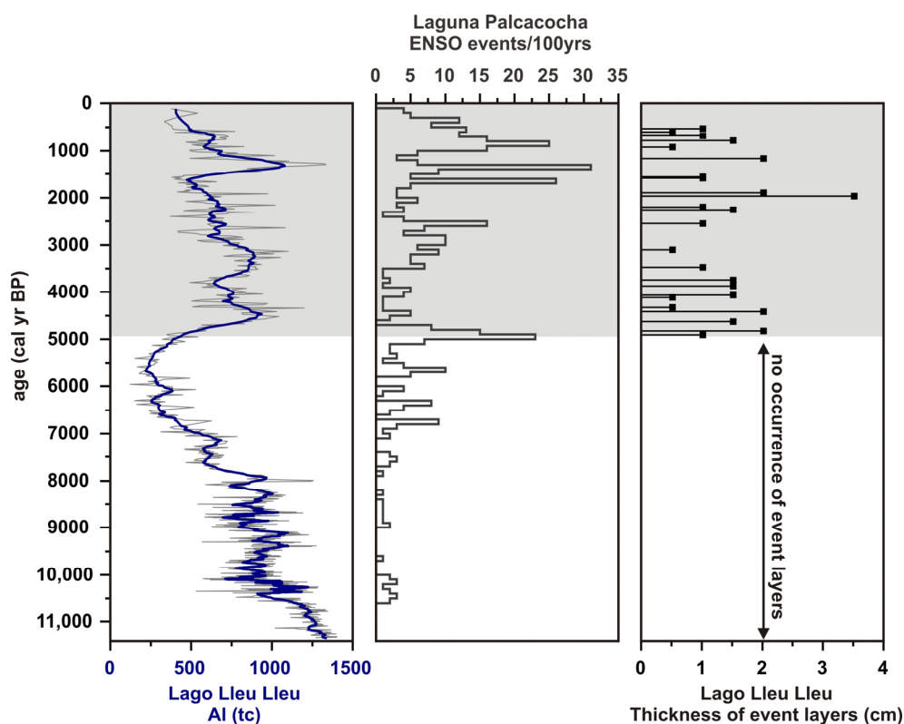
Figure 4.7: Comparison of the aluminium intensities measured on the Lleu Lleu sediments, reflecting detrital input (left), the number of ENSO events per 100 years observed in sediments of Laguna Pallcacocha, Southern Ecuador (Moy et al., 2002) (middle), and the temporal occurrence and thickness of event layers found in the Lleu Lleu sediments (right). Thick solid line of the Al-record displays the 11-point moving average. Highlighted in grey are the last 5000 years during which ENSO events are more frequent and event layers became apparent.
