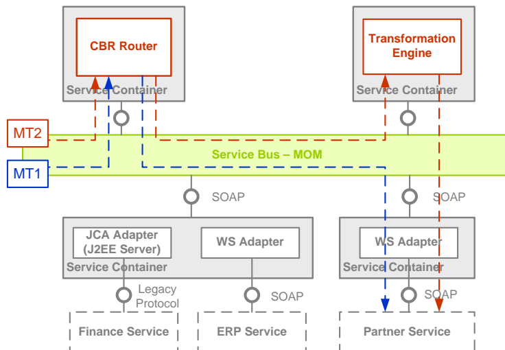
Figure 12: Content-based routing in an ESB.
