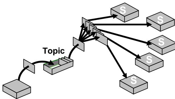
Figure 3: publish/subscribe-messaging architecture [8]
