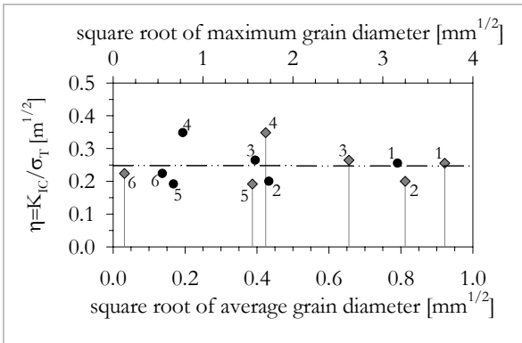
Fig. 6-6. Ratio of Mode I fracture toughness and tensile strength, \eta , as a function of square root of grain diameter, dg . \eta remains constant irrespective of dg . Grey diamonds indicate average grain diameter, black cycles designate maximum grain diameter. 1 Äspö diorite, 2 Aue granite, 3 Mizunami granite, 4 Carrara marble, 5 Flechtingen sandstone, 6 Rüdersdorf limestone.
