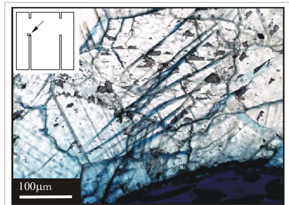
Fig. 5-20. Micrograph of the bottom notch at \sim 99\% of the maximum axial stress in Carrara marble. Only en échelon cracks are visible.
