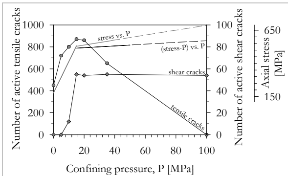
Fig. 5-30. Compilation of data from Kemeny (1993). Grey solid line indicates strength envelope (axial stress, \sigma , vs. confining pressure, P ); black solid line indicates (\sigma-P) vs. P . Dashed lines indicate extrapolation. Circles: active tensile cracks; diamonds: active shear cracks. Refer to text for discussion.
