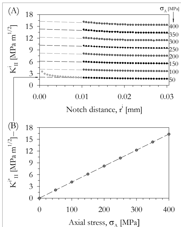
Fig. 5-5. Displacement Extrapolation Technique. (A) K_{II}^i as determined from the displacements calculated by FEM as function of the distance from the notch tip, r_i . Extrapolation to r = 0 for determination of axis intercept K_{II}^{i*} is indicated by dashed lines for increasing axial loads, \sigma_A , at constant confining pressure, P , of 5 MPa. (B) K_{II}^{i*} as determined from (A) as function of \sigma_A . The obtained stress intensity factor increases linearly with increase in axial load. Elastic properties of Mizunami granite.
