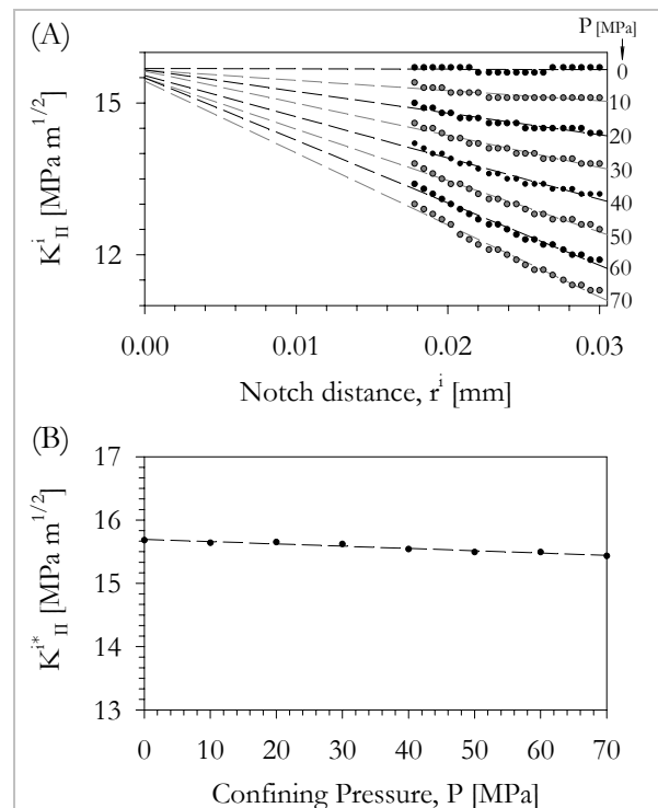
Fig. 5-6. Displacement Extrapolation Technique. (A) K_{II}^i as determined from the displacements calculated by FEM as function of the distance from the notch tip, r_i . Extrapolation to r = 0 for determination of axis intercept K_{II}^{i*} is indicated by dashed lines for increasing confining pressure, P , at constant axial load, \sigma_A , of 400 MPa. (B) Influence of confining pressure on K_{II}^{i*} at \sigma_A = 400 MPa. Elastic properties of Mizunami granite; corresponding plots for other rock types are given in Appendix E.
