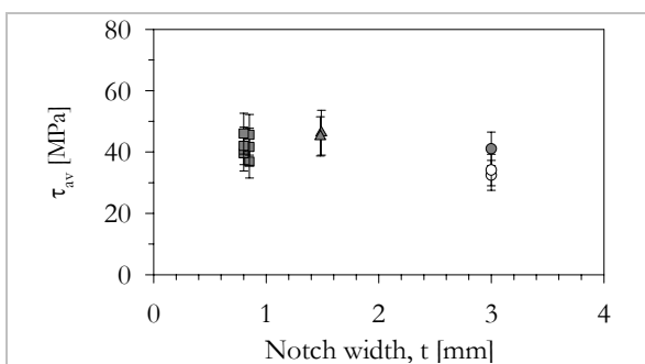
Fig. 5-13. Influence of the notch width, t , on \tau_{av} for Carrara marble. The shear stress at failure – calculated for the outer notch diameter – remains similar for the tested t . [White circles: W=50mm, D=50mm, a≈5mm, ID≈25mm, IP≈15 mm, t≈3mm; Grey circles: W=50mm, D=50mm, a≈5mm, ID≈22mm, IP≈15 mm, t≈3mm; grey triangles: W=50mm, D=50mm, a≈5mm, ID≈25mm, IP≈15 mm, t≈1.5mm; grey squares: W=25mm, D=50mm, a≈5mm, ID≈25mm, IP≈15 mm, t≈0.8mm].
